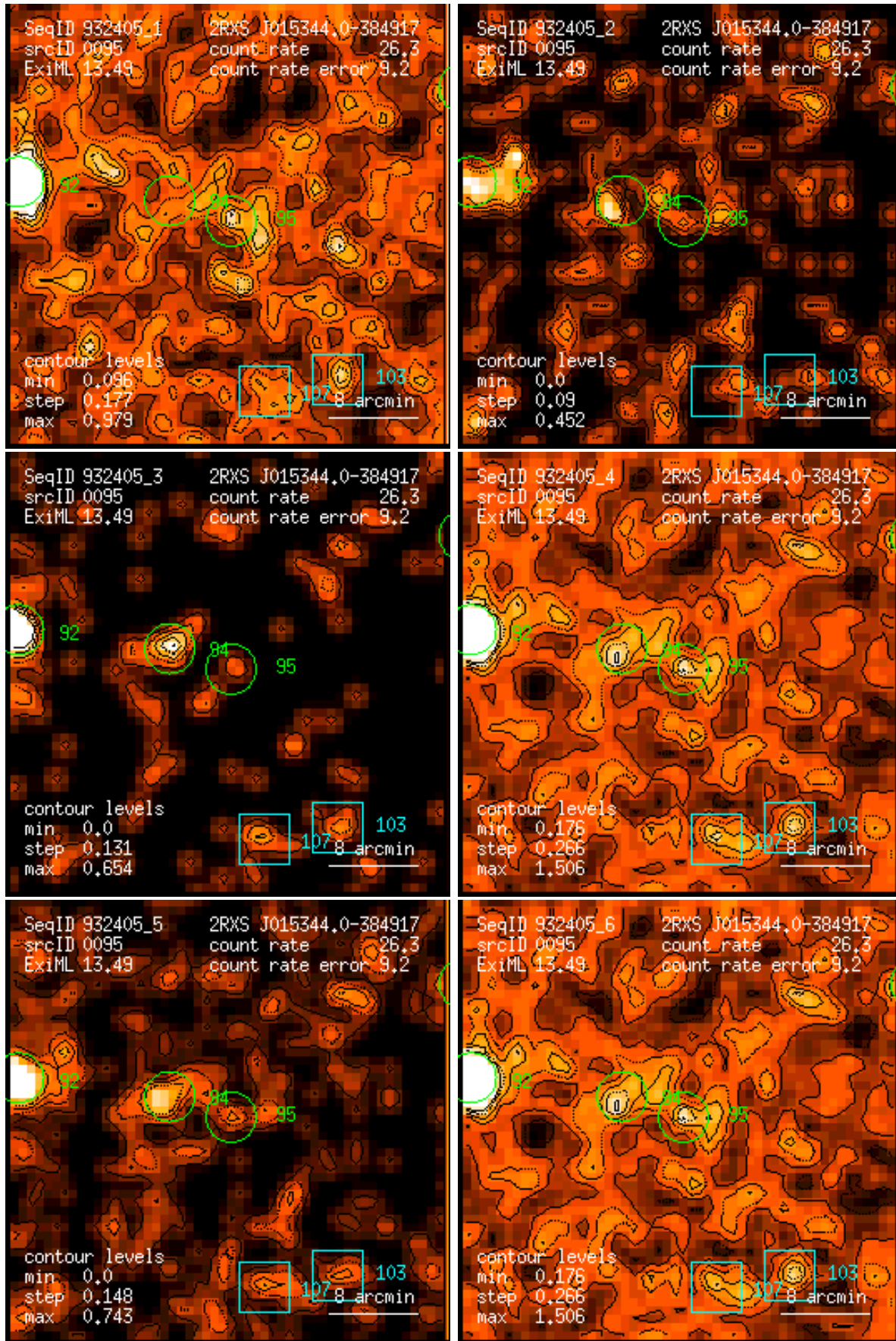
Figure 95: RASS 932405: detection 0095: band rate images, Gaussian filter: (1) PSPC channels 11 – 41, (2) 52 – 90, (3) 91 – 201, (4) 11 – 235, (5) 52 – 201, (6) 11 – 201. Broad band rates in counts/ks. Band rate contour levels in counts/ks/arcmin 2 .
