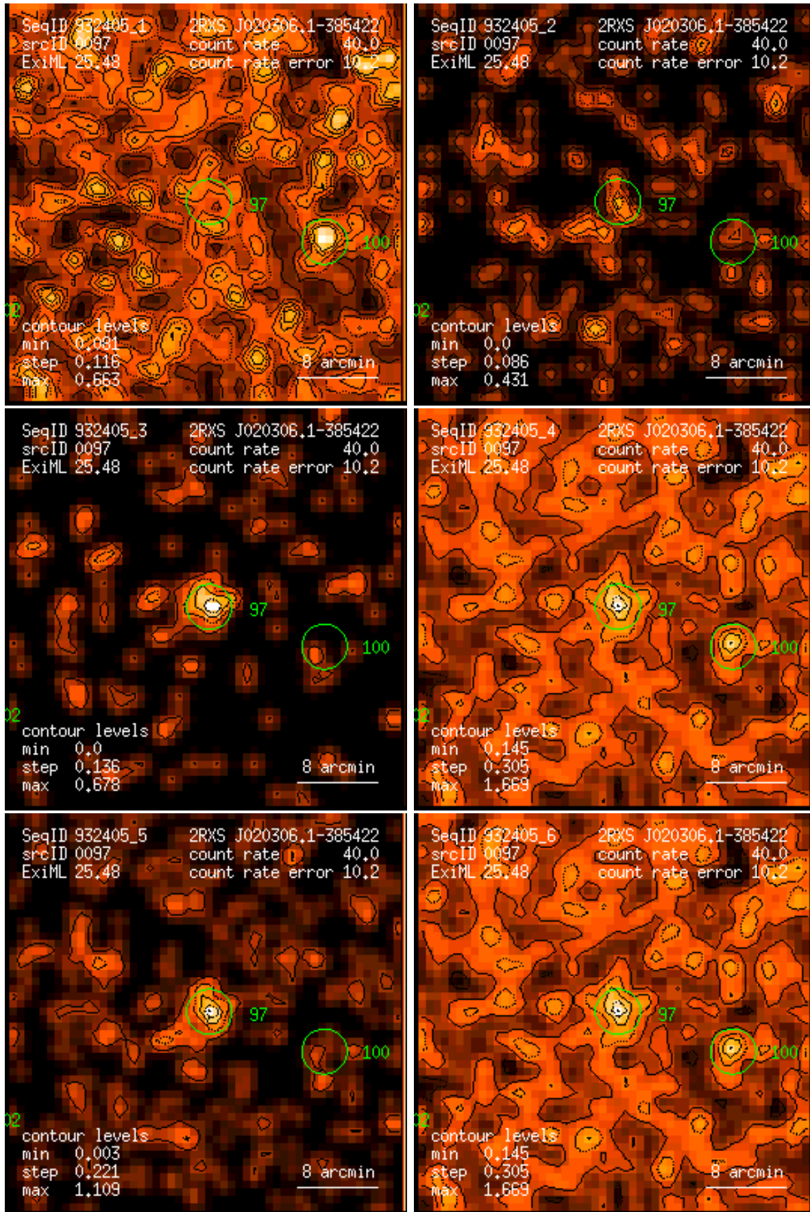
Figure 97: RASS 932405: detection 0097: band rate images, Gaussian filter: (1) PSPC channels 11 – 41, (2) 52 – 90, (3) 91 – 201, (4) 11 – 235, (5) 52 – 201, (6) 11 – 201. Broad band rates in counts/ks. Band rate contour levels in counts/ks/arcmin 2 .
