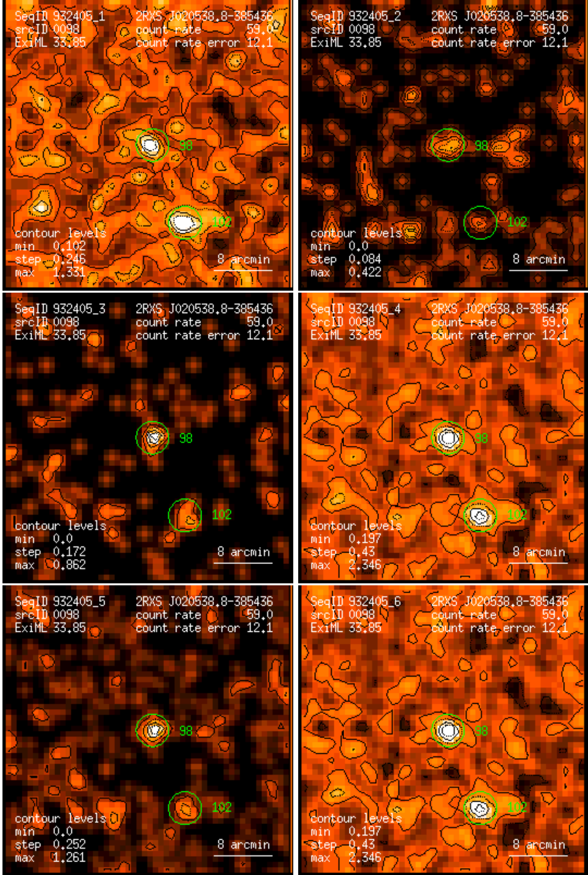
Figure 98: RASS 932405: detection 0098: band rate images, Gaussian filter: (1) PSPC channels 11 – 41, (2) 52 – 90, (3) 91 – 201, (4) 11 – 235, (5) 52 – 201, (6) 11 – 201. Broad band rates in counts/ks. Band rate contour levels in counts/ks/arcmin 2 .
