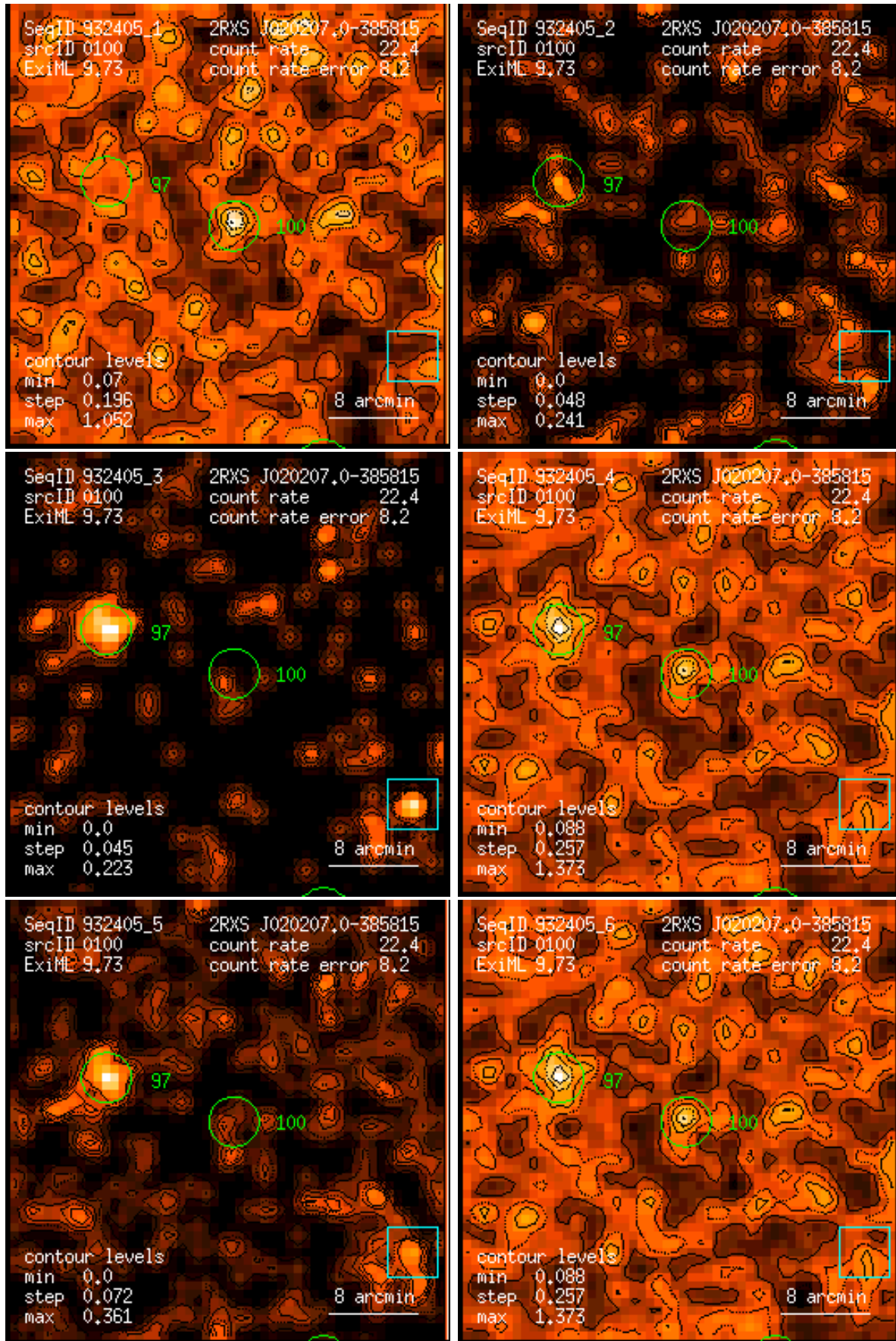
Figure 100: RASS 932405: detection 0100: band rate images, Gaussian filter: (1) PSPC channels 11 – 41, (2) 52 – 90, (3) 91 – 201, (4) 11 – 235, (5) 52 – 201, (6) 11 – 201. Broad band rates in counts/ks. Band rate contour levels in counts/ks/arcmin 2 .
