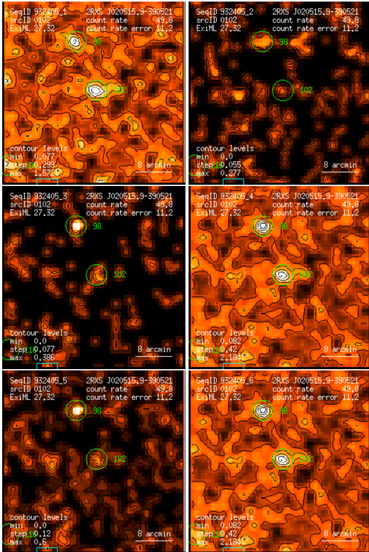
Figure 102: RASS 932405: detection 0102: band rate images, Gaussian filter: (1) PSPC channels 11 – 41, (2) 52 – 90, (3) 91 – 201, (4) 11 – 235, (5) 52 – 201, (6) 11 – 201. Broad band rates in counts/ks. Band rate contour levels in counts/ks/arcmin 2 .
