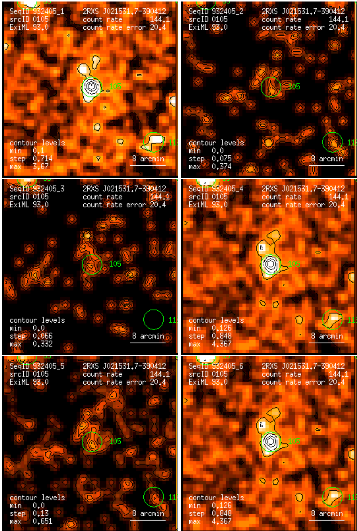
Figure 105: RASS 932405: detection 0105: band rate images, Gaussian filter: (1) PSPC channels 11 – 41, (2) 52 – 90, (3) 91 – 201, (4) 11 – 235, (5) 52 – 201, (6) 11 – 201. Broad band rates in counts/ks. Band rate contour levels in counts/ks/arcmin 2 .
