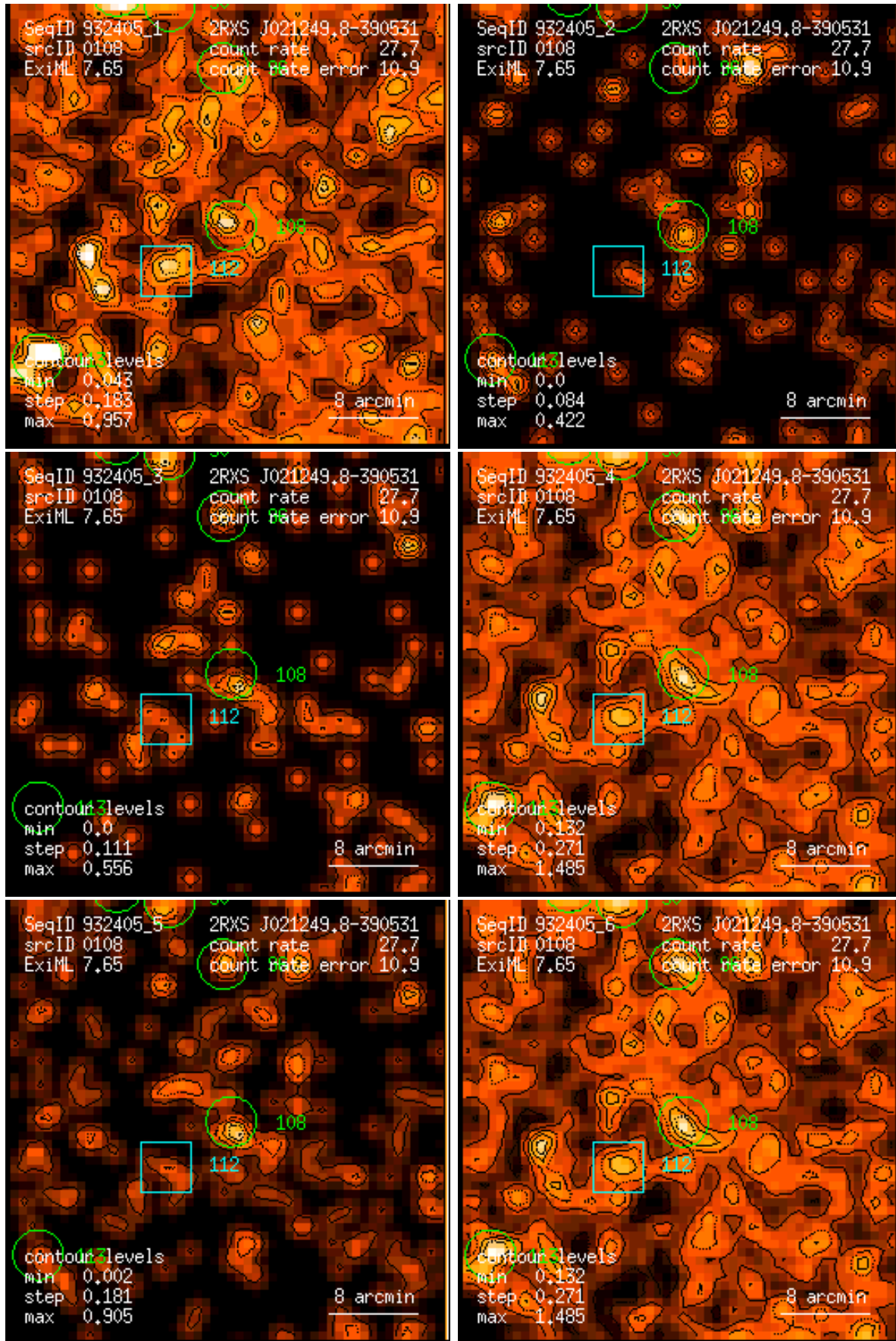
Figure 108: RASS 932405: detection 0108: band rate images, Gaussian filter: (1) PSPC channels 11 – 41, (2) 52 – 90, (3) 91 – 201, (4) 11 – 235, (5) 52 – 201, (6) 11 – 201. Broad band rates in counts/ks. Band rate contour levels in counts/ks/arcmin 2 .
