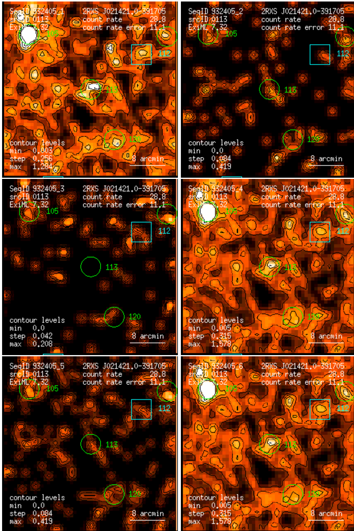
Figure 113: RASS 932405: detection 0113: band rate images, Gaussian filter: (1) PSPC channels 11 – 41, (2) 52 – 90, (3) 91 – 201, (4) 11 – 235, (5) 52 – 201, (6) 11 – 201. Broad band rates in counts/ks. Band rate contour levels in counts/ks/arcmin 2 .
