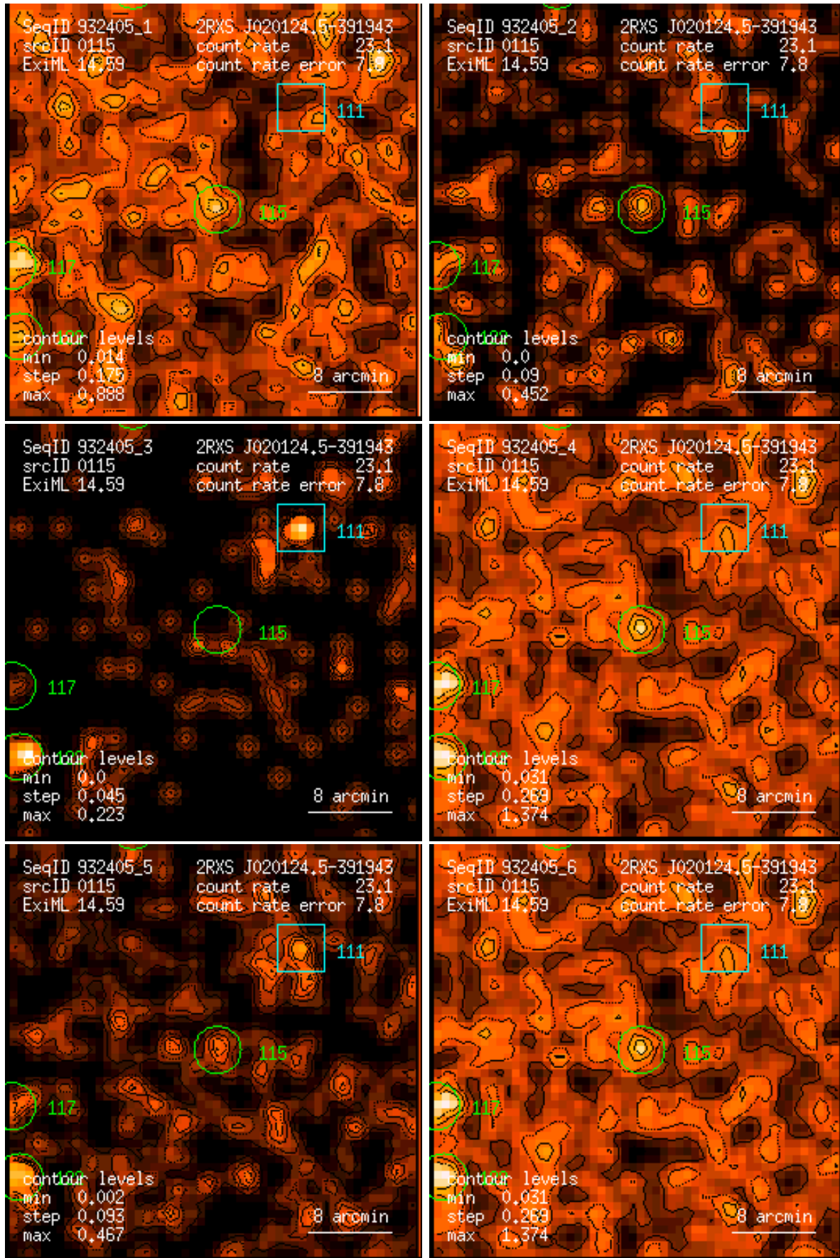
Figure 115: RASS 932405: detection 0115: band rate images, Gaussian filter: (1) PSPC channels 11 – 41, (2) 52 – 90, (3) 91 – 201, (4) 11 – 235, (5) 52 – 201, (6) 11 – 201. Broad band rates in counts/ks. Band rate contour levels in counts/ks/arcmin 2 .
