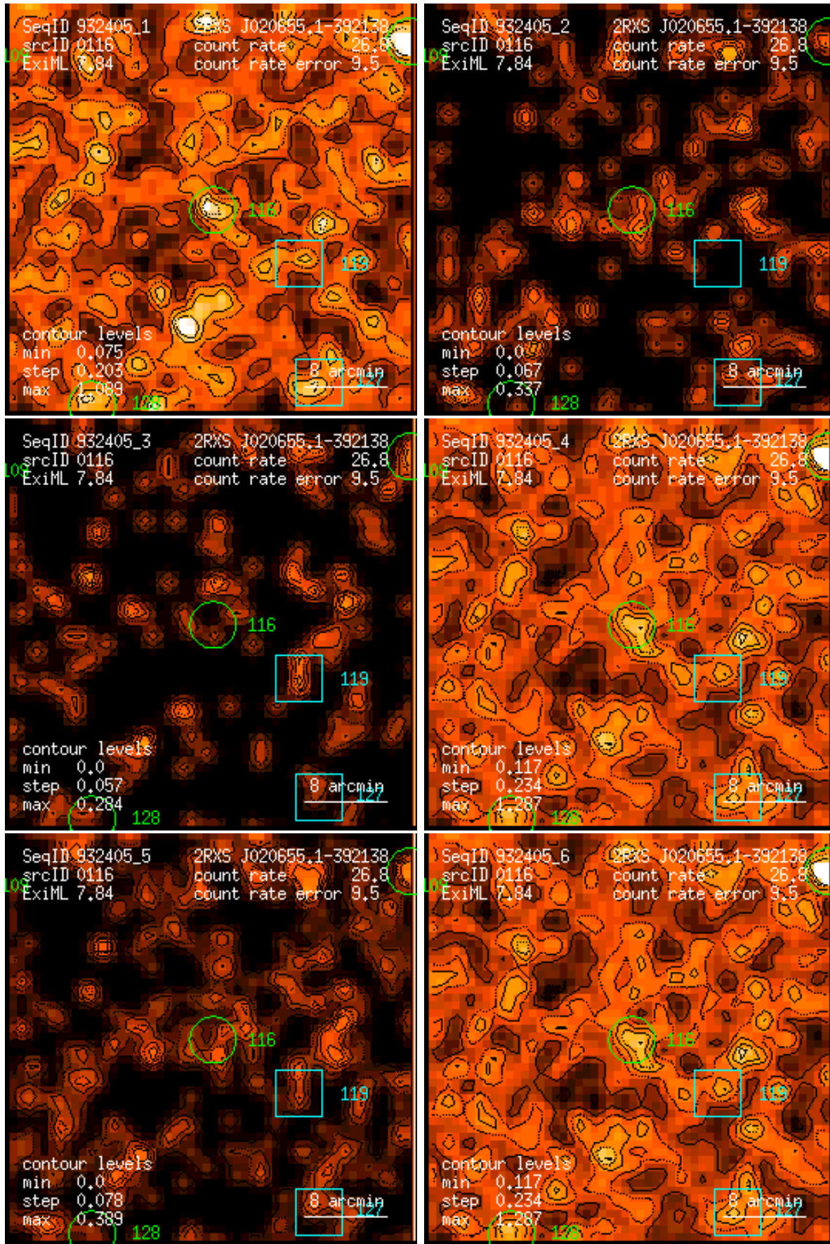
Figure 116: RASS 932405: detection 0116: band rate images, Gaussian filter: (1) PSPC channels 11 – 41, (2) 52 – 90, (3) 91 – 201, (4) 11 – 235, (5) 52 – 201, (6) 11 – 201. Broad band rates in counts/ks. Band rate contour levels in counts/ks/arcmin 2 .
