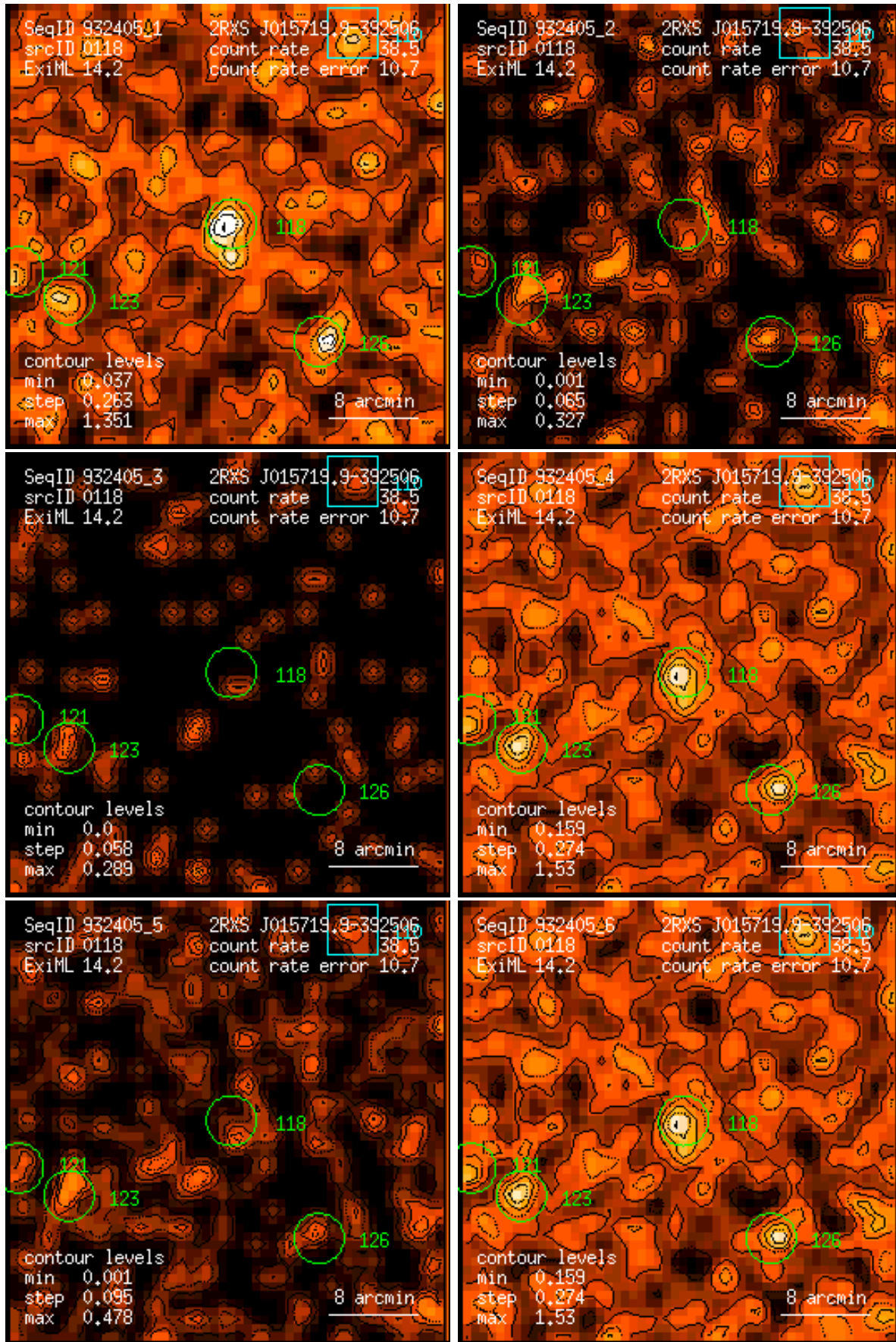
Figure 118: RASS 932405: detection 0118: band rate images, Gaussian filter: (1) PSPC channels 11 – 41, (2) 52 – 90, (3) 91 – 201, (4) 11 – 235, (5) 52 – 201, (6) 11 – 201. Broad band rates in counts/ks. Band rate contour levels in counts/ks/arcmin 2 .
