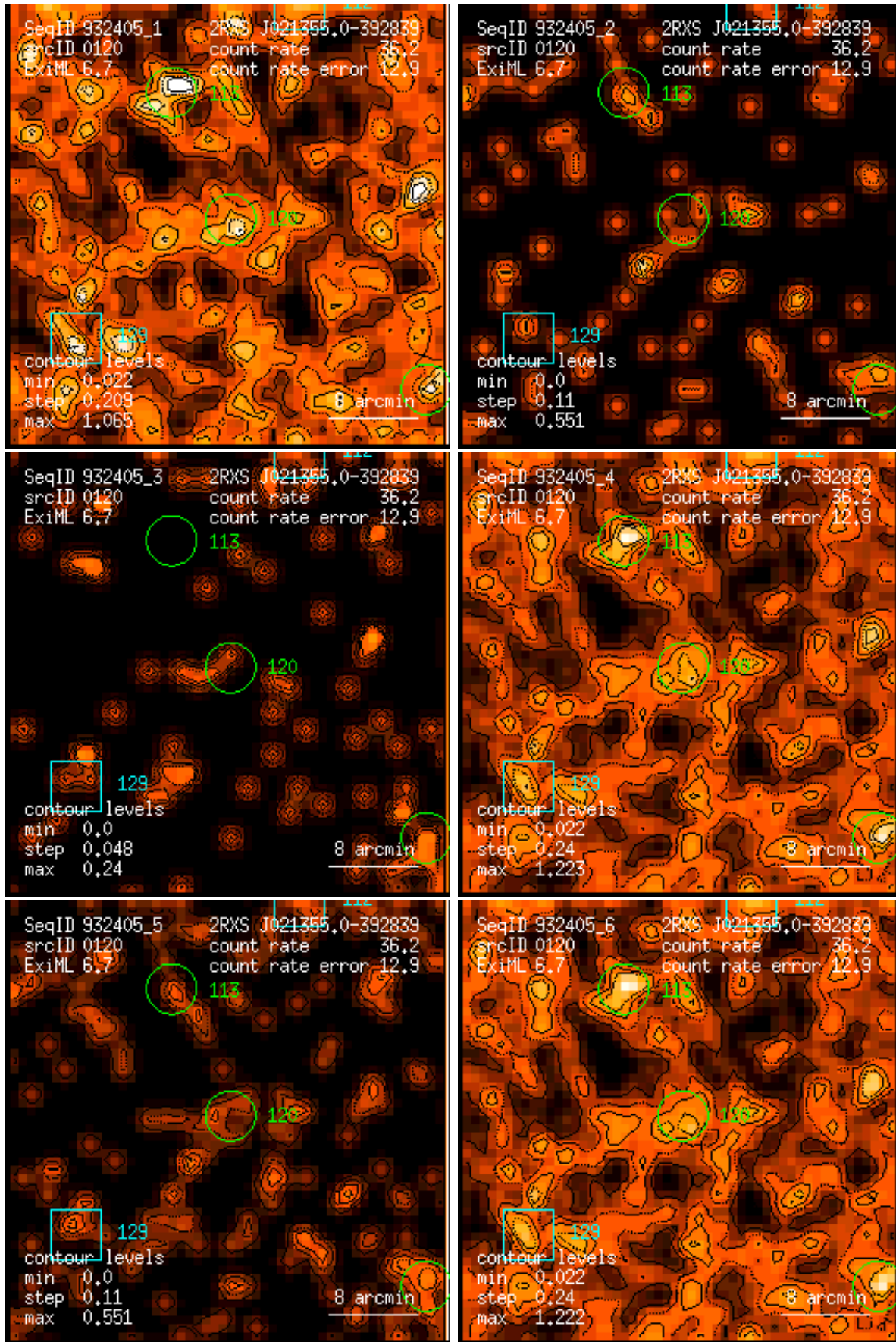
Figure 120: RASS 932405: detection 0120: band rate images, Gaussian filter: (1) PSPC channels 11 – 41, (2) 52 – 90, (3) 91 – 201, (4) 11 – 235, (5) 52 – 201, (6) 11 – 201. Broad band rates in counts/ks. Band rate contour levels in counts/ks/arcmin 2 .
