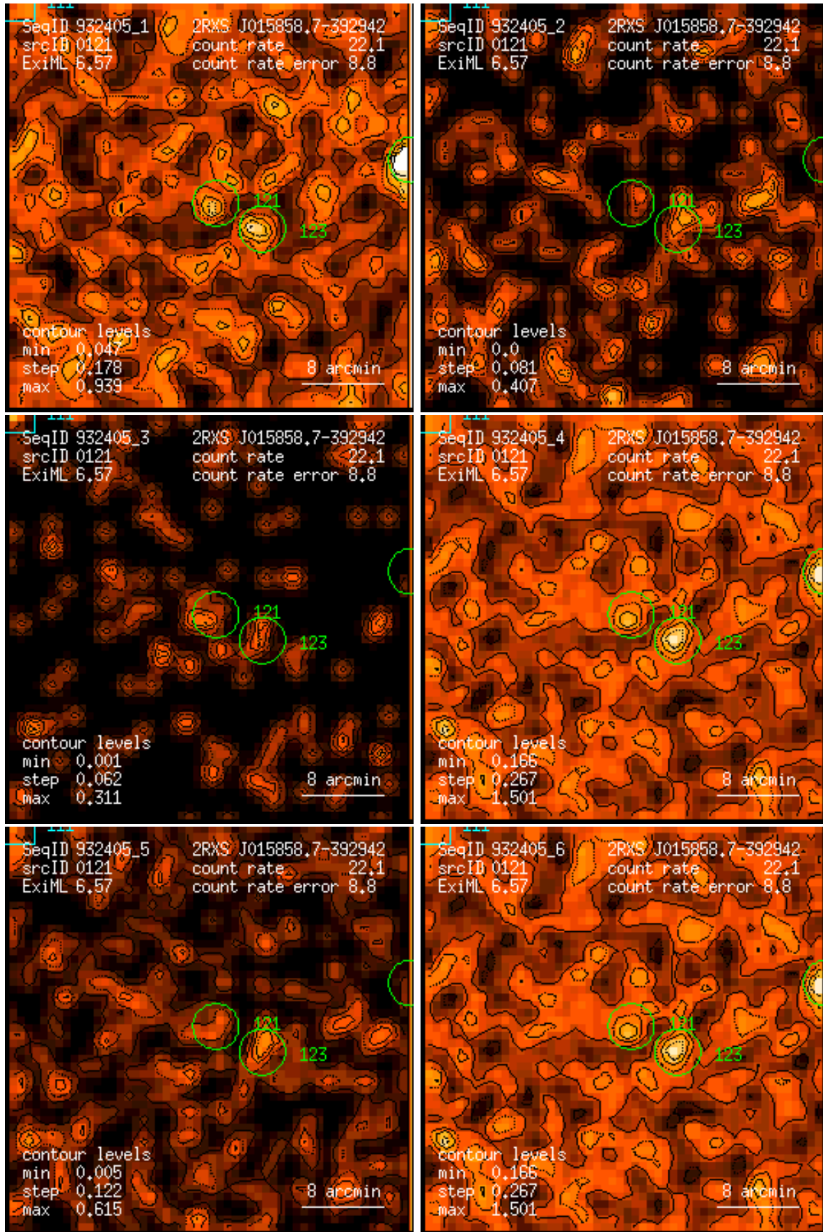
Figure 121: RASS 932405: detection 0121: band rate images, Gaussian filter: (1) PSPC channels 11 – 41, (2) 52 – 90, (3) 91 – 201, (4) 11 – 235, (5) 52 – 201, (6) 11 – 201. Broad band rates in counts/ks. Band rate contour levels in counts/ks/arcmin 2 .
