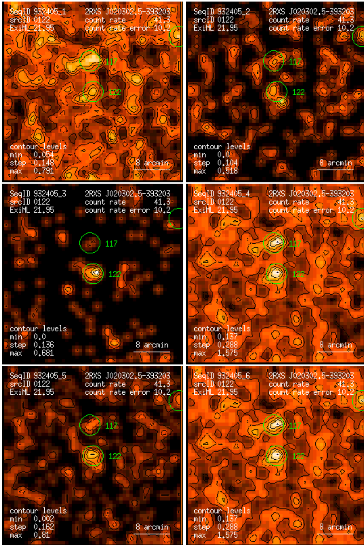
Figure 122: RASS 932405: detection 0122: band rate images, Gaussian filter: (1) PSPC channels 11 – 41, (2) 52 – 90, (3) 91 – 201, (4) 11 – 235, (5) 52 – 201, (6) 11 – 201. Broad band rates in counts/ks. Band rate contour levels in counts/ks/arcmin 2 .
