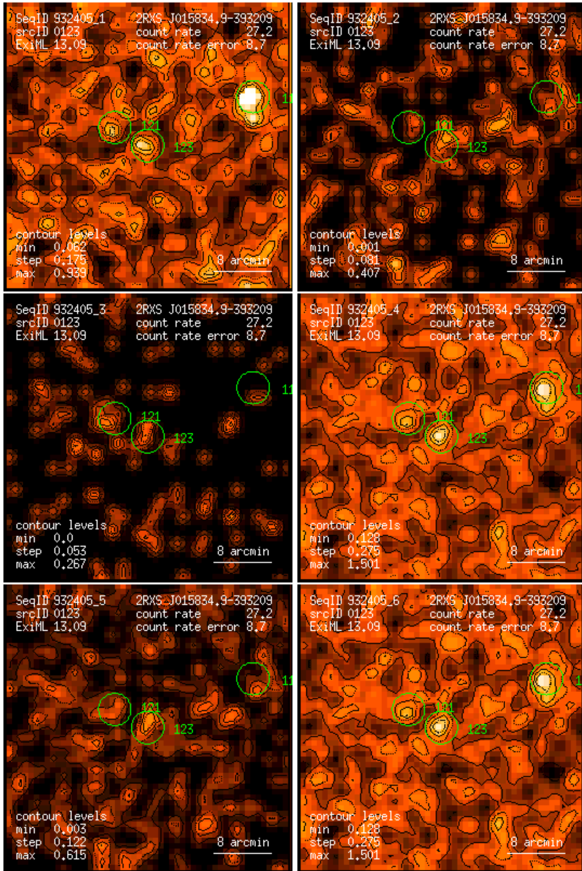
Figure 123: RASS 932405: detection 0123: band rate images, Gaussian filter: (1) PSPC channels 11 – 41, (2) 52 – 90, (3) 91 – 201, (4) 11 – 235, (5) 52 – 201, (6) 11 – 201. Broad band rates in counts/ks. Band rate contour levels in counts/ks/arcmin 2 .
