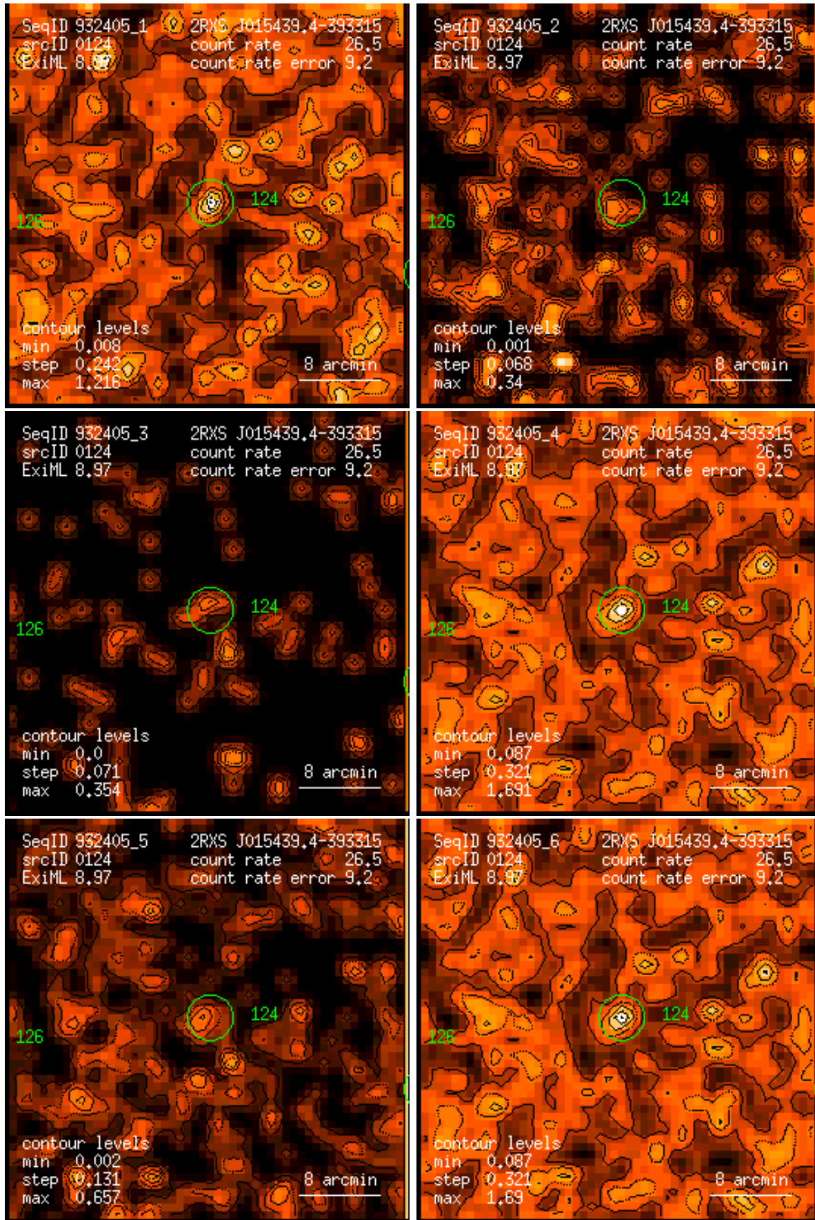
Figure 124: RASS 932405: detection 0124: band rate images, Gaussian filter: (1) PSPC channels 11 – 41, (2) 52 – 90, (3) 91 – 201, (4) 11 – 235, (5) 52 – 201, (6) 11 – 201. Broad band rates in counts/ks. Band rate contour levels in counts/ks/arcmin 2 .
