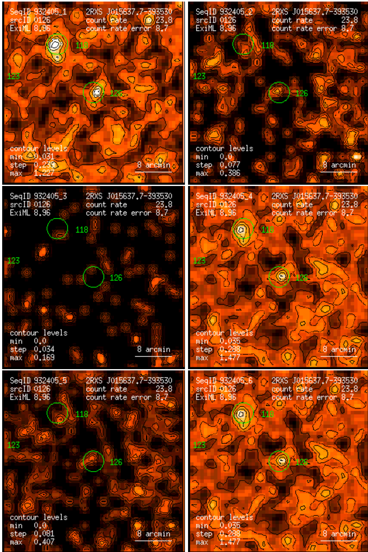
Figure 126: RASS 932405: detection 0126: band rate images, Gaussian filter: (1) PSPC channels 11 – 41, (2) 52 – 90, (3) 91 – 201, (4) 11 – 235, (5) 52 – 201, (6) 11 – 201. Broad band rates in counts/ks. Band rate contour levels in counts/ks/arcmin 2 .
