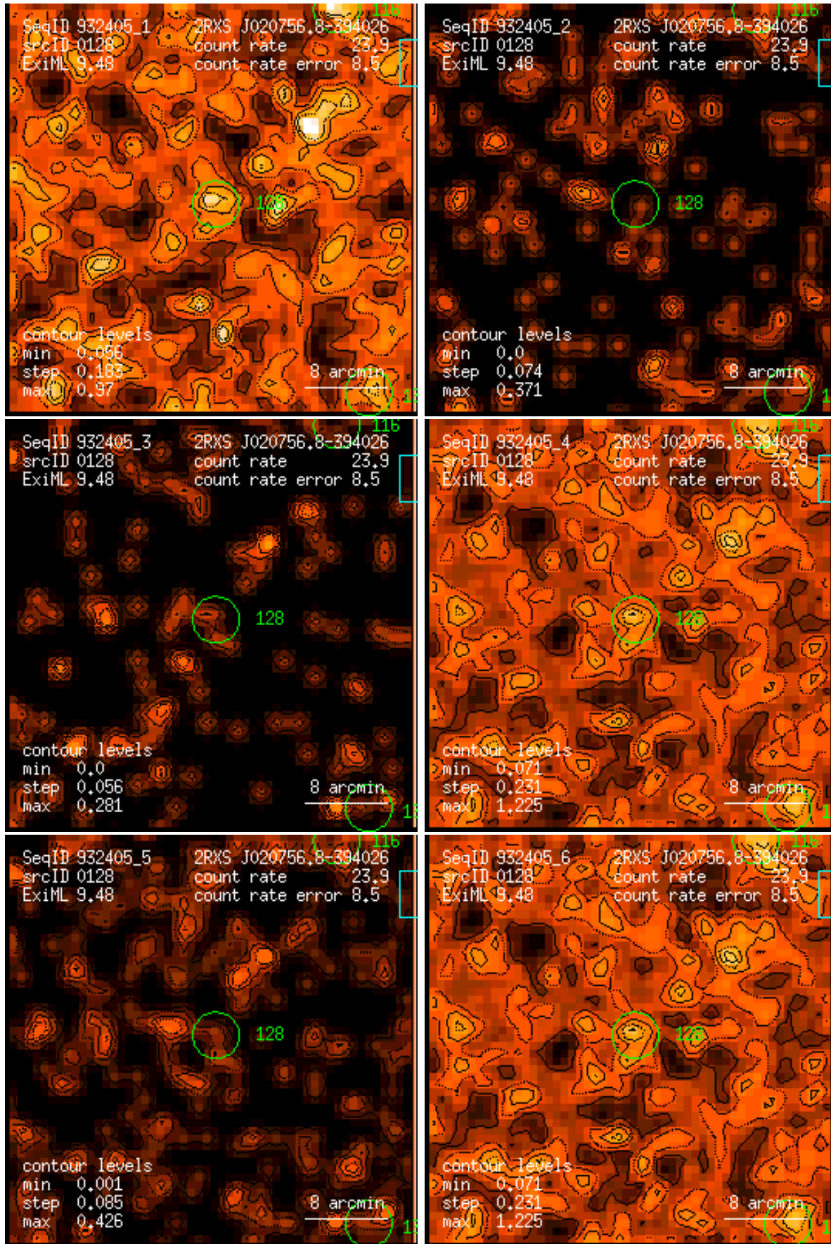
Figure 128: RASS 932405: detection 0128: band rate images, Gaussian filter: (1) PSPC channels 11 – 41, (2) 52 – 90, (3) 91 – 201, (4) 11 – 235, (5) 52 – 201, (6) 11 – 201. Broad band rates in counts/ks. Band rate contour levels in counts/ks/arcmin 2 .
