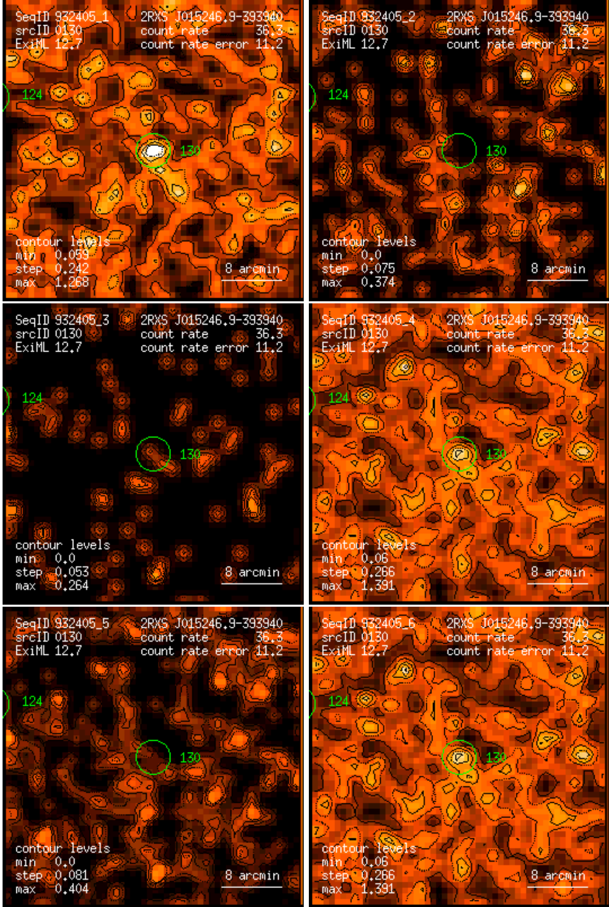
Figure 130: RASS 932405: detection 0130: band rate images, Gaussian filter: (1) PSPC channels 11 – 41, (2) 52 – 90, (3) 91 – 201, (4) 11 – 235, (5) 52 – 201, (6) 11 – 201. Broad band rates in counts/ks. Band rate contour levels in counts/ks/arcmin 2 .
