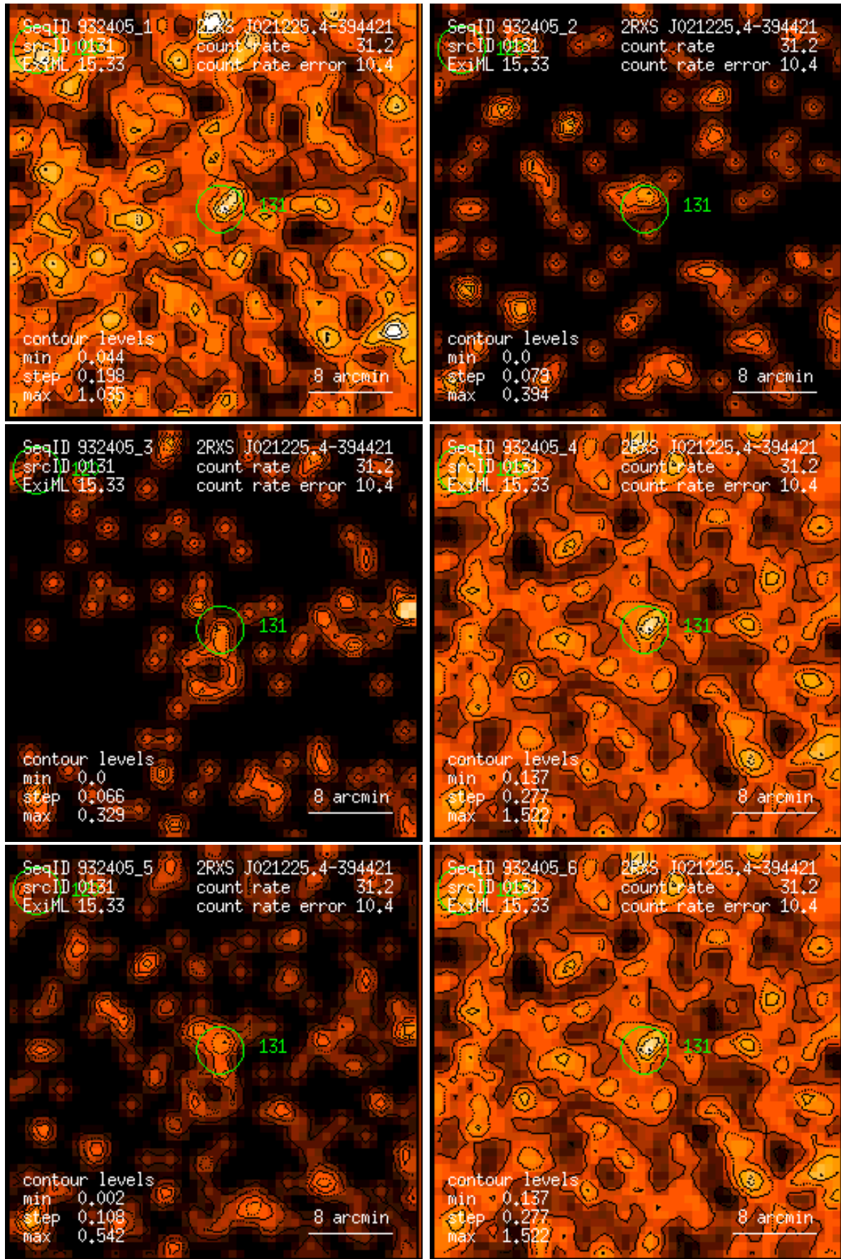
Figure 131: RASS 932405: detection 0131: band rate images, Gaussian filter: (1) PSPC channels 11 – 41, (2) 52 – 90, (3) 91 – 201, (4) 11 – 235, (5) 52 – 201, (6) 11 – 201. Broad band rates in counts/ks. Band rate contour levels in counts/ks/arcmin 2 .
