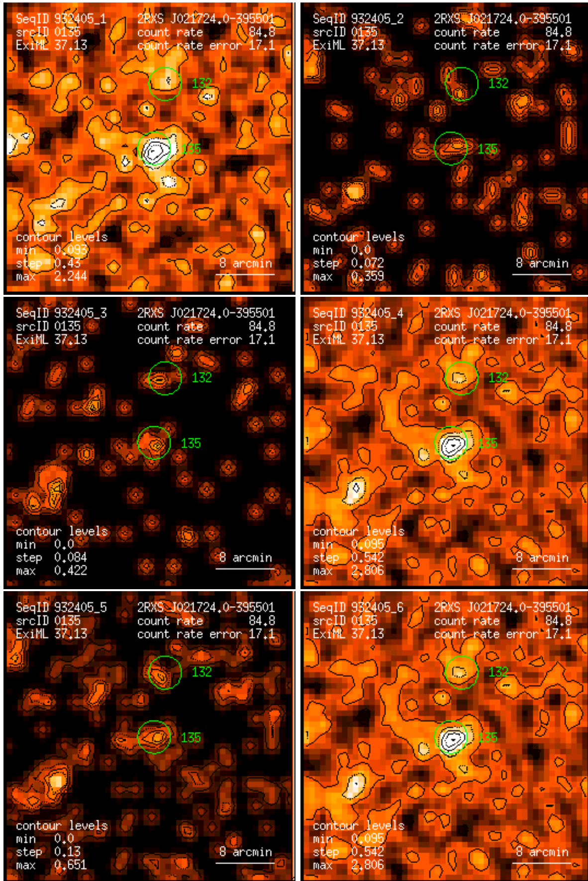
Figure 135: RASS 932405: detection 0135: band rate images, Gaussian filter: (1) PSPC channels 11 – 41, (2) 52 – 90, (3) 91 – 201, (4) 11 – 235, (5) 52 – 201, (6) 11 – 201. Broad band rates in counts/ks. Band rate contour levels in counts/ks/arcmin 2 .
