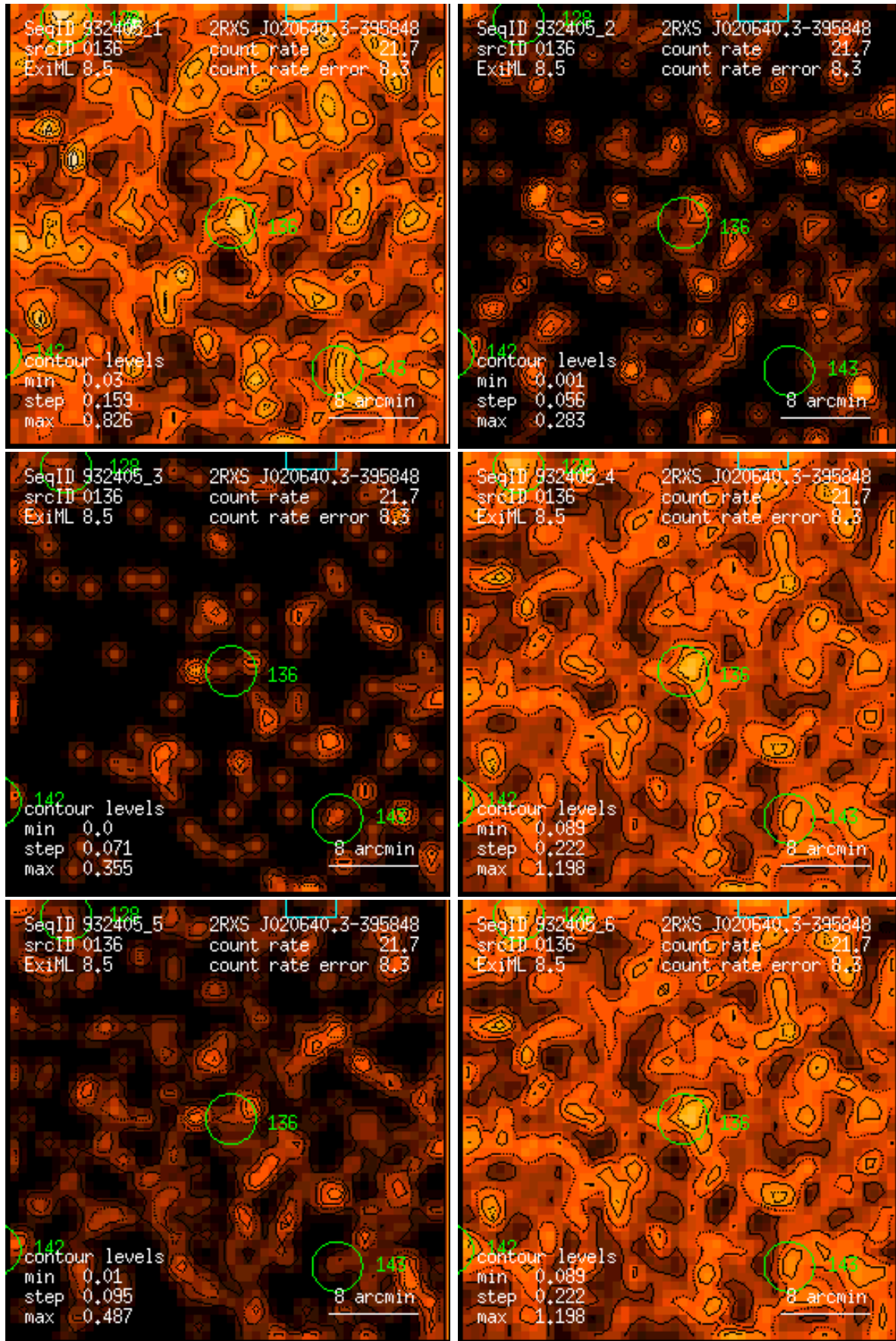
Figure 136: RASS 932405: detection 0136: band rate images, Gaussian filter: (1) PSPC channels 11 – 41, (2) 52 – 90, (3) 91 – 201, (4) 11 – 235, (5) 52 – 201, (6) 11 – 201. Broad band rates in counts/ks. Band rate contour levels in counts/ks/arcmin 2 .
