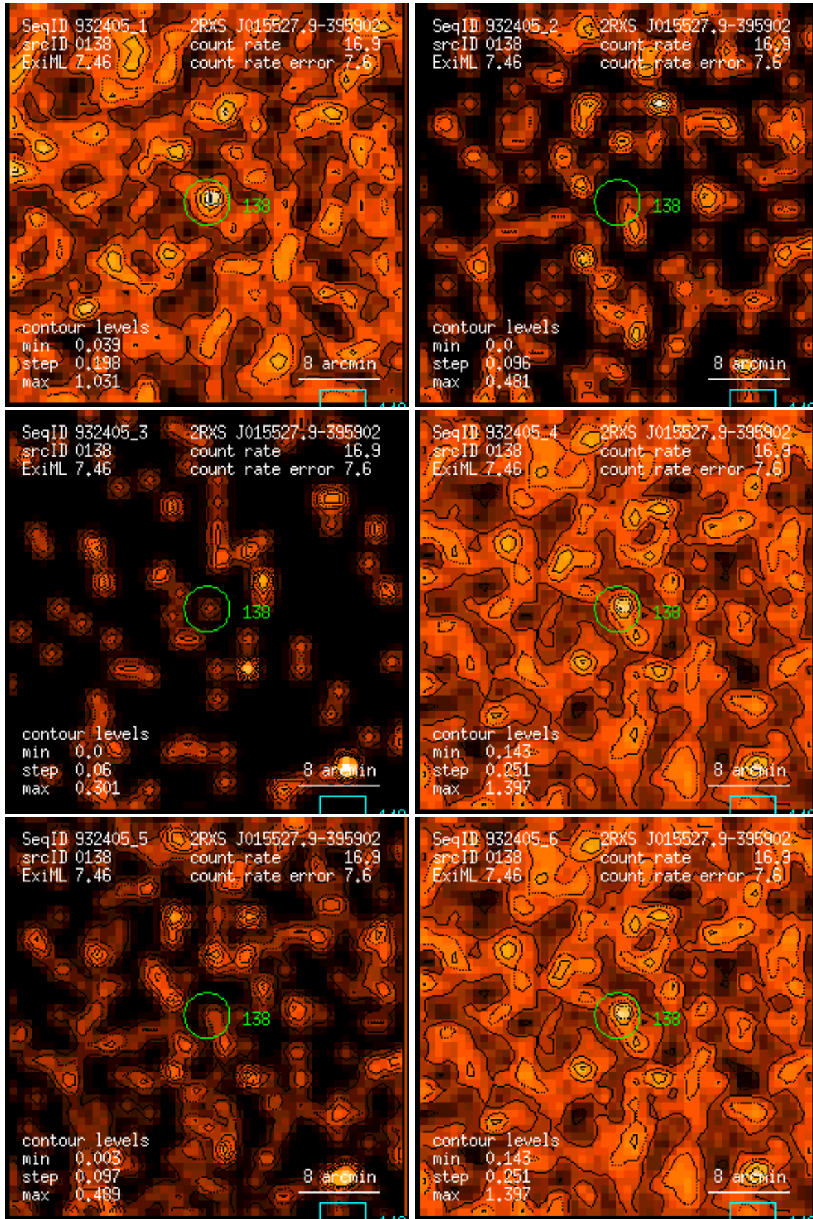
Figure 138: RASS 932405: detection 0138: band rate images, Gaussian filter: (1) PSPC channels 11 – 41, (2) 52 – 90, (3) 91 – 201, (4) 11 – 235, (5) 52 – 201, (6) 11 – 201. Broad band rates in counts/ks. Band rate contour levels in counts/ks/arcmin 2 .
