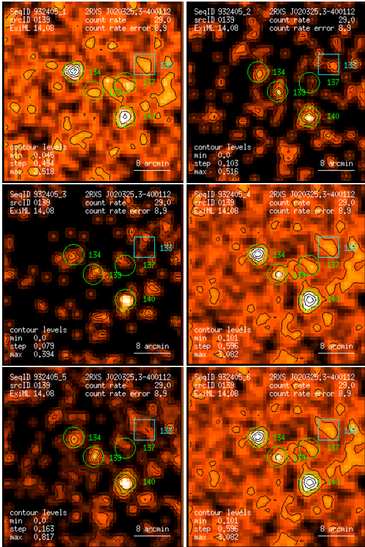
Figure 139: RASS 932405: detection 0139: band rate images, Gaussian filter: (1) PSPC channels 11 – 41, (2) 52 – 90, (3) 91 – 201, (4) 11 – 235, (5) 52 – 201, (6) 11 – 201. Broad band rates in counts/ks. Band rate contour levels in counts/ks/arcmin 2 .
