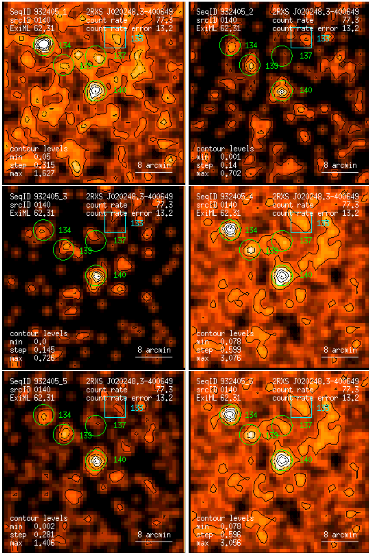
Figure 140: RASS 932405: detection 0140: band rate images, Gaussian filter: (1) PSPC channels 11 – 41, (2) 52 – 90, (3) 91 – 201, (4) 11 – 235, (5) 52 – 201, (6) 11 – 201. Broad band rates in counts/ks. Band rate contour levels in counts/ks/arcmin 2 .
