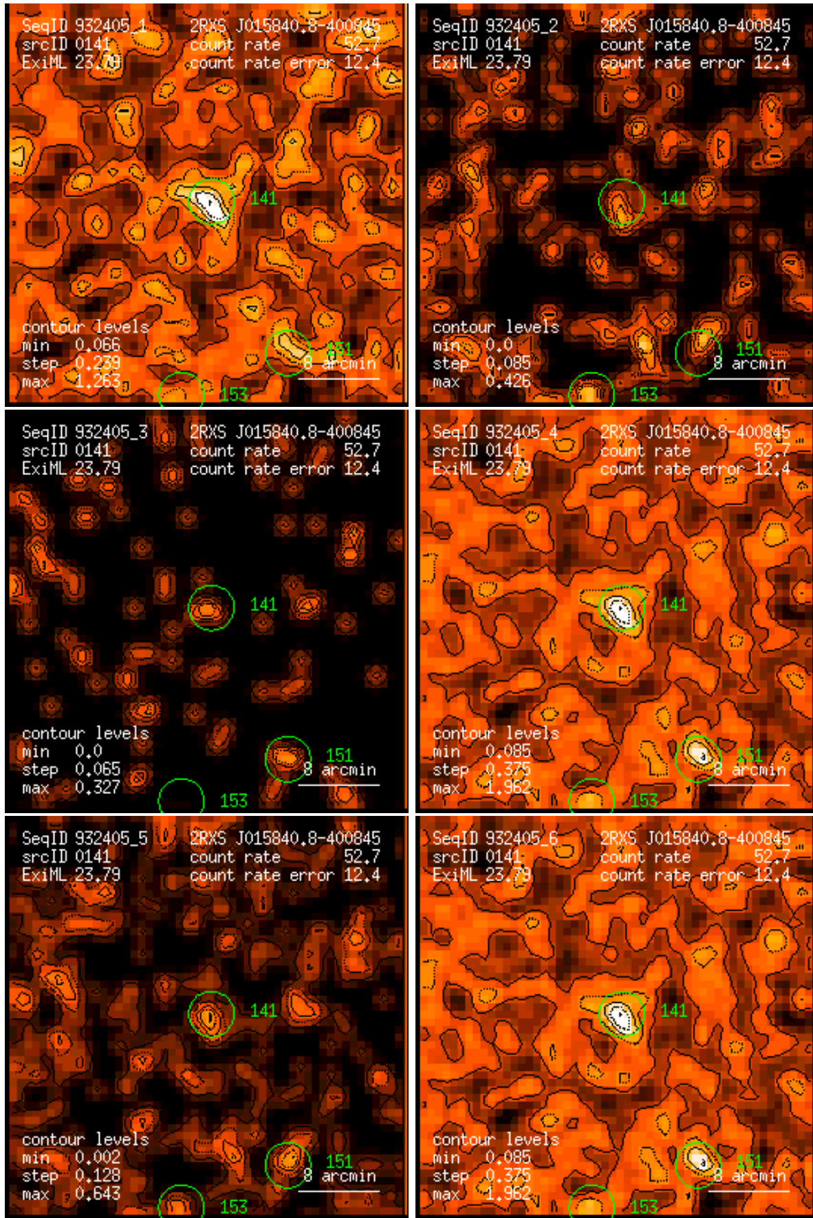
Figure 141: RASS 932405: detection 0141: band rate images, Gaussian filter: (1) PSPC channels 11 – 41, (2) 52 – 90, (3) 91 – 201, (4) 11 – 235, (5) 52 – 201, (6) 11 – 201. Broad band rates in counts/ks. Band rate contour levels in counts/ks/arcmin 2 .
