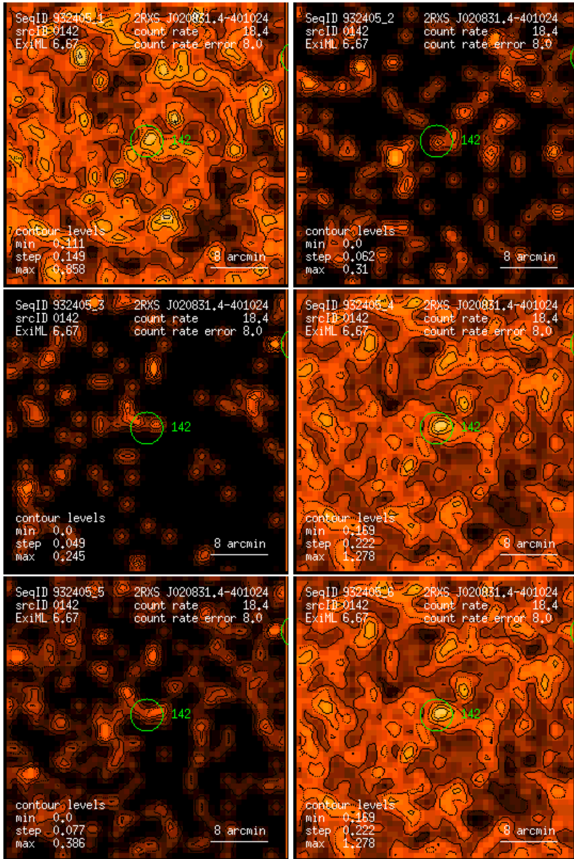
Figure 142: RASS 932405: detection 0142: band rate images, Gaussian filter: (1) PSPC channels 11 – 41, (2) 52 – 90, (3) 91 – 201, (4) 11 – 235, (5) 52 – 201, (6) 11 – 201. Broad band rates in counts/ks. Band rate contour levels in counts/ks/arcmin 2 .
