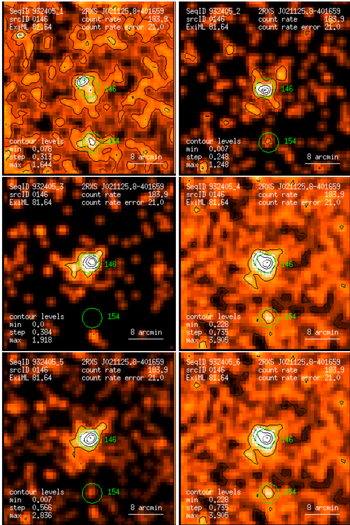
Figure 146: RASS 932405: detection 0146: band rate images, Gaussian filter: (1) PSPC channels 11 – 41, (2) 52 – 90, (3) 91 – 201, (4) 11 – 235, (5) 52 – 201, (6) 11 – 201. Broad band rates in counts/ks. Band rate contour levels in counts/ks/arcmin 2 .
