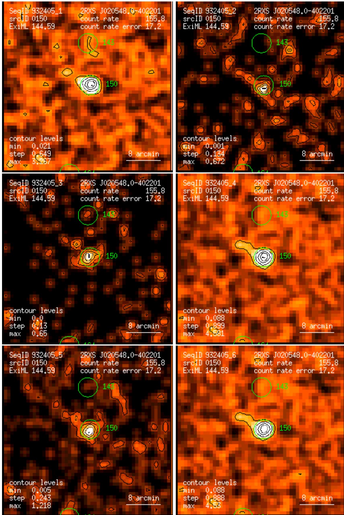
Figure 150: RASS 932405: detection 0150: band rate images, Gaussian filter: (1) PSPC channels 11 – 41, (2) 52 – 90, (3) 91 – 201, (4) 11 – 235, (5) 52 – 201, (6) 11 – 201. Broad band rates in counts/ks. Band rate contour levels in counts/ks/arcmin 2 .
