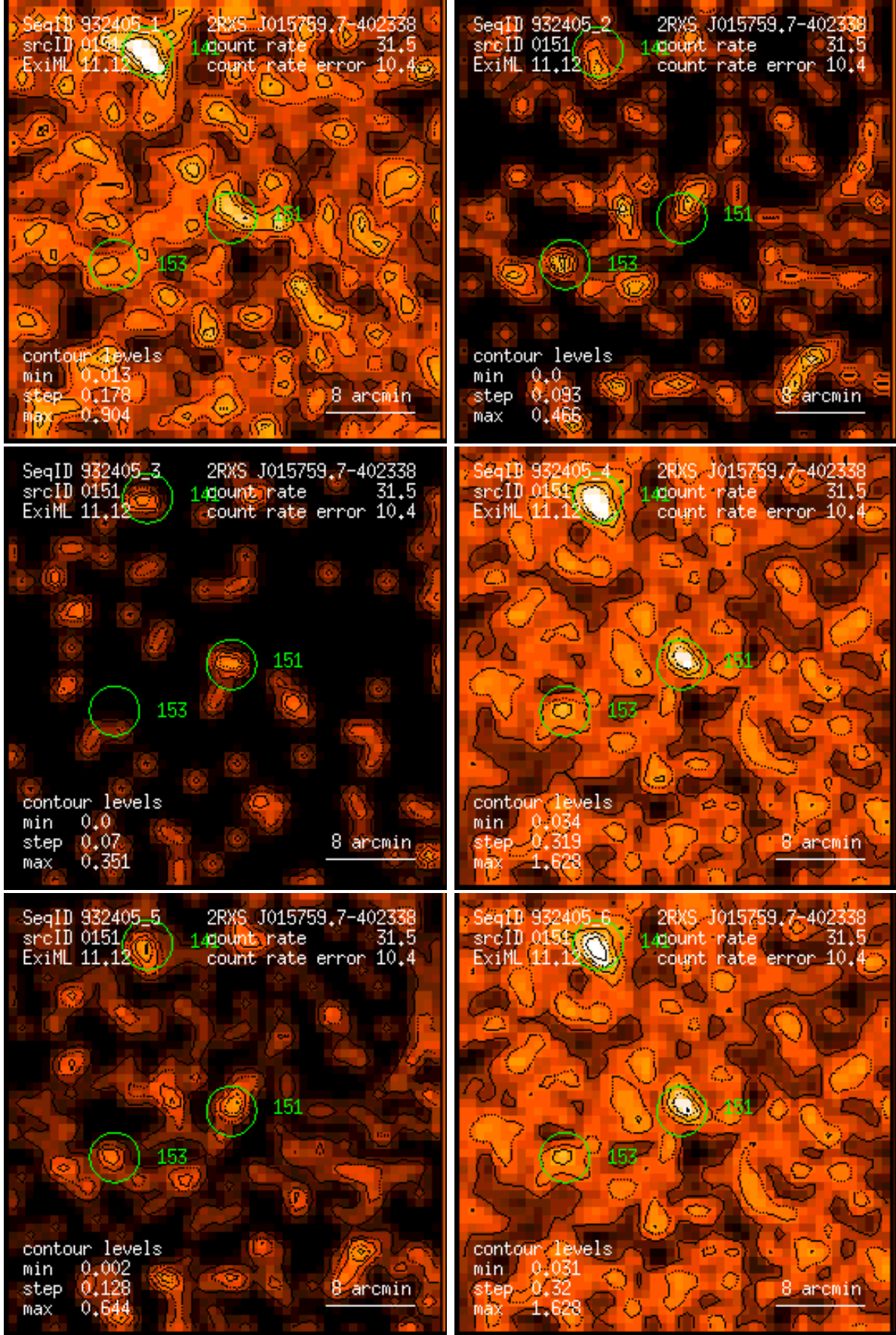
Figure 151: RASS 932405: detection 0151: band rate images, Gaussian filter: (1) PSPC channels 11 – 41, (2) 52 – 90, (3) 91 – 201, (4) 11 – 235, (5) 52 – 201, (6) 11 – 201. Broad band rates in counts/ks. Band rate contour levels in counts/ks/arcmin 2 .
