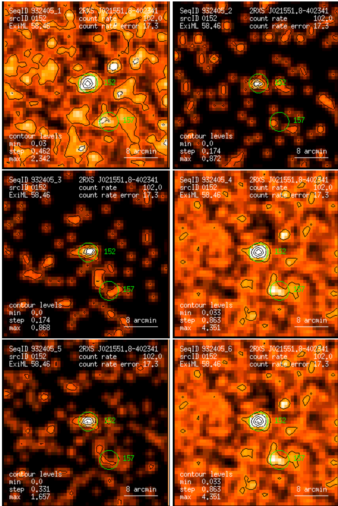
Figure 152: RASS 932405: detection 0152: band rate images, Gaussian filter: (1) PSPC channels 11 – 41, (2) 52 – 90, (3) 91 – 201, (4) 11 – 235, (5) 52 – 201, (6) 11 – 201. Broad band rates in counts/ks. Band rate contour levels in counts/ks/arcmin 2 .
