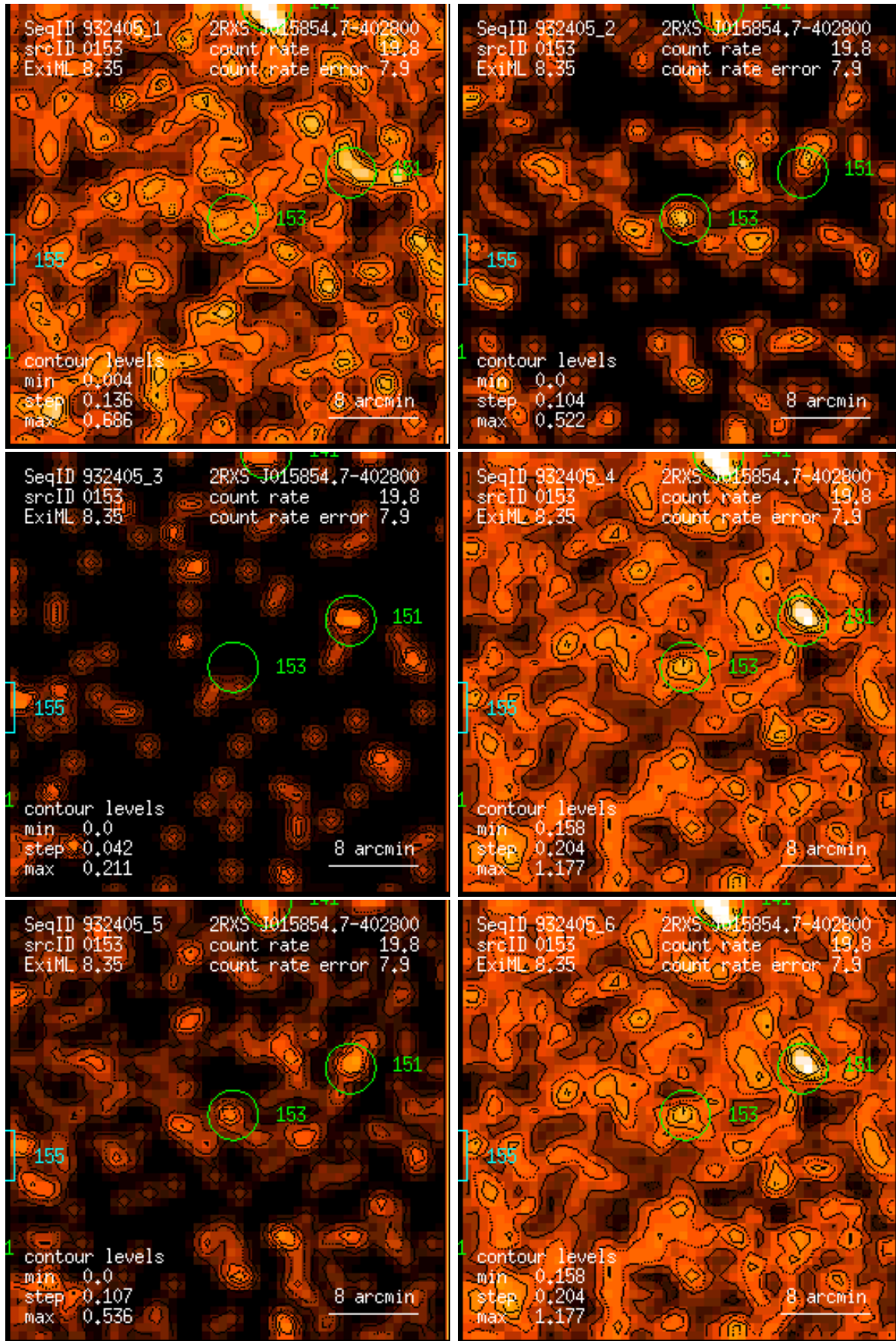
Figure 153: RASS 932405: detection 0153: band rate images, Gaussian filter: (1) PSPC channels 11 – 41, (2) 52 – 90, (3) 91 – 201, (4) 11 – 235, (5) 52 – 201, (6) 11 – 201. Broad band rates in counts/ks. Band rate contour levels in counts/ks/arcmin 2 .
