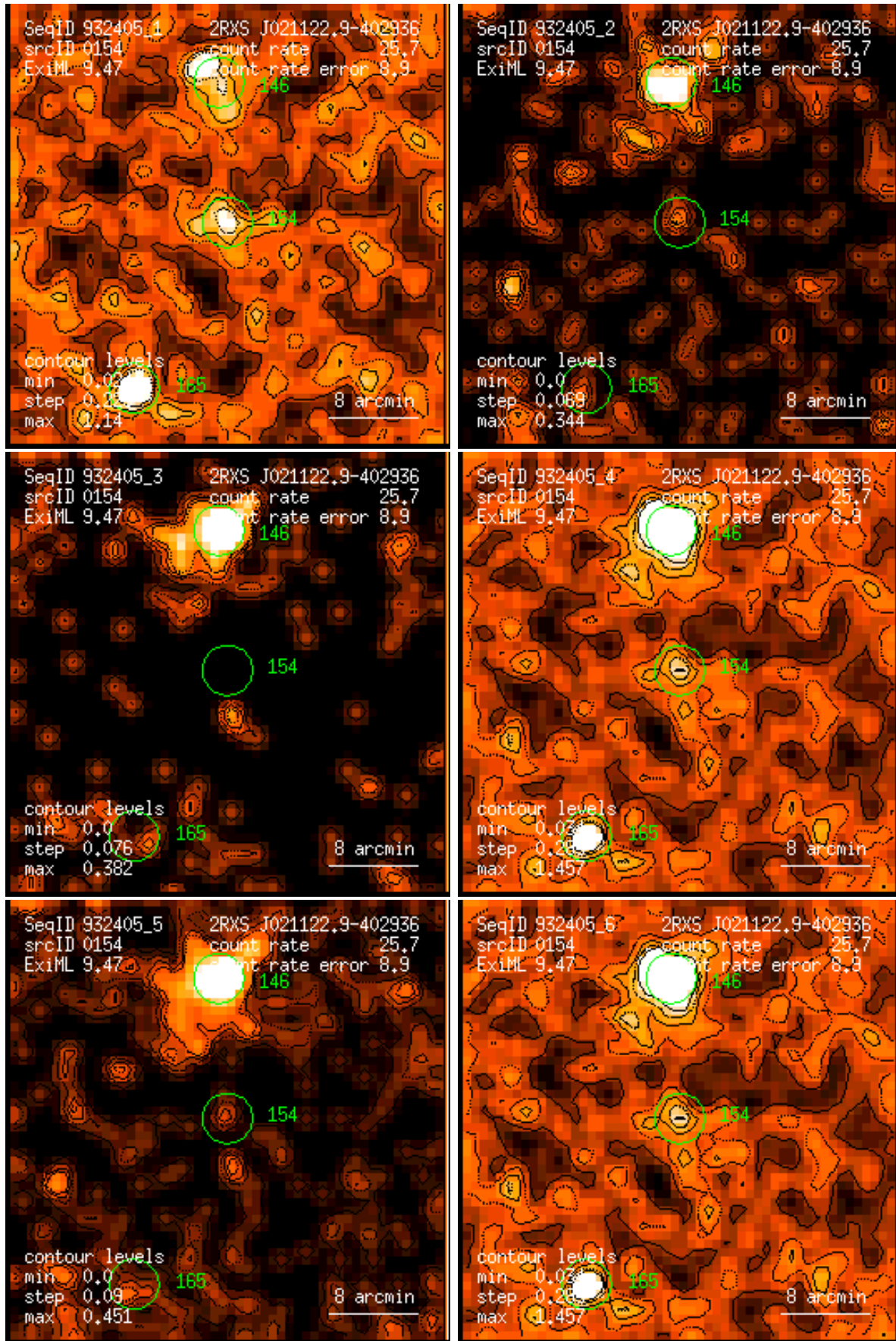
Figure 154: RASS 932405: detection 0154: band rate images, Gaussian filter: (1) PSPC channels 11 – 41, (2) 52 – 90, (3) 91 – 201, (4) 11 – 235, (5) 52 – 201, (6) 11 – 201. Broad band rates in counts/ks. Band rate contour levels in counts/ks/arcmin 2 .
