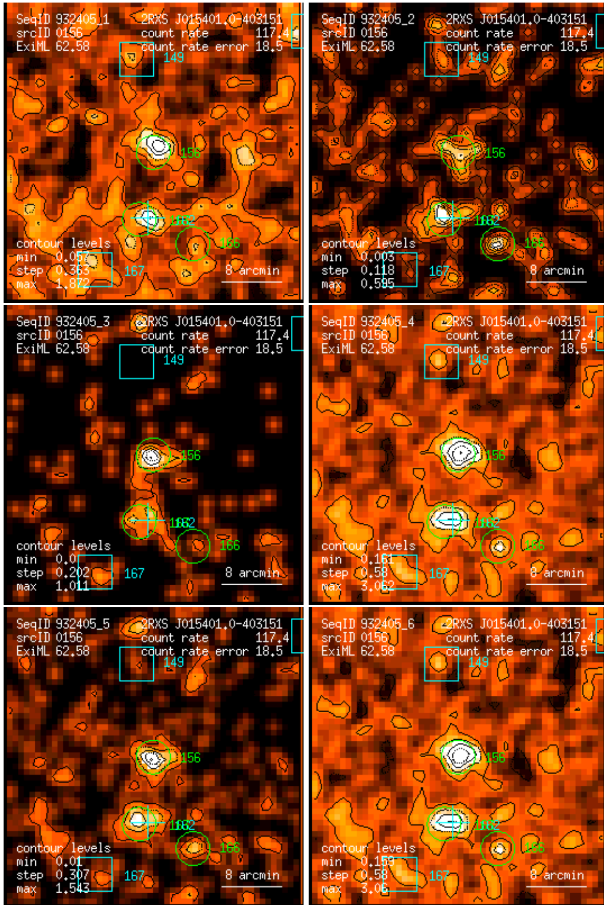
Figure 156: RASS 932405: detection 0156: band rate images, Gaussian filter: (1) PSPC channels 11 – 41, (2) 52 – 90, (3) 91 – 201, (4) 11 – 235, (5) 52 – 201, (6) 11 – 201. Broad band rates in counts/ks. Band rate contour levels in counts/ks/arcmin 2 .
