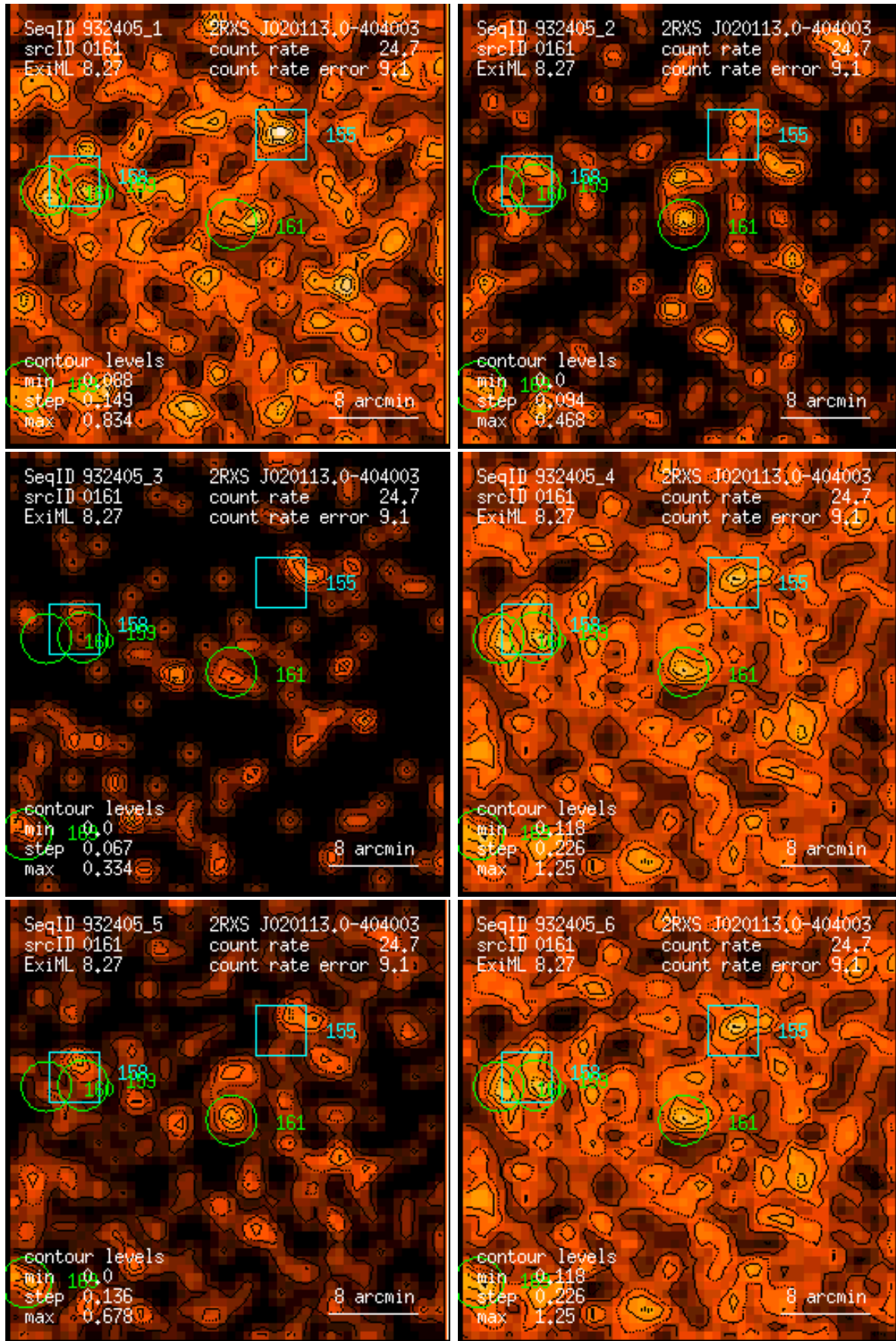
Figure 161: RASS 932405: detection 0161: band rate images, Gaussian filter: (1) PSPC channels 11 – 41, (2) 52 – 90, (3) 91 – 201, (4) 11 – 235, (5) 52 – 201, (6) 11 – 201. Broad band rates in counts/ks. Band rate contour levels in counts/ks/arcmin 2 .
