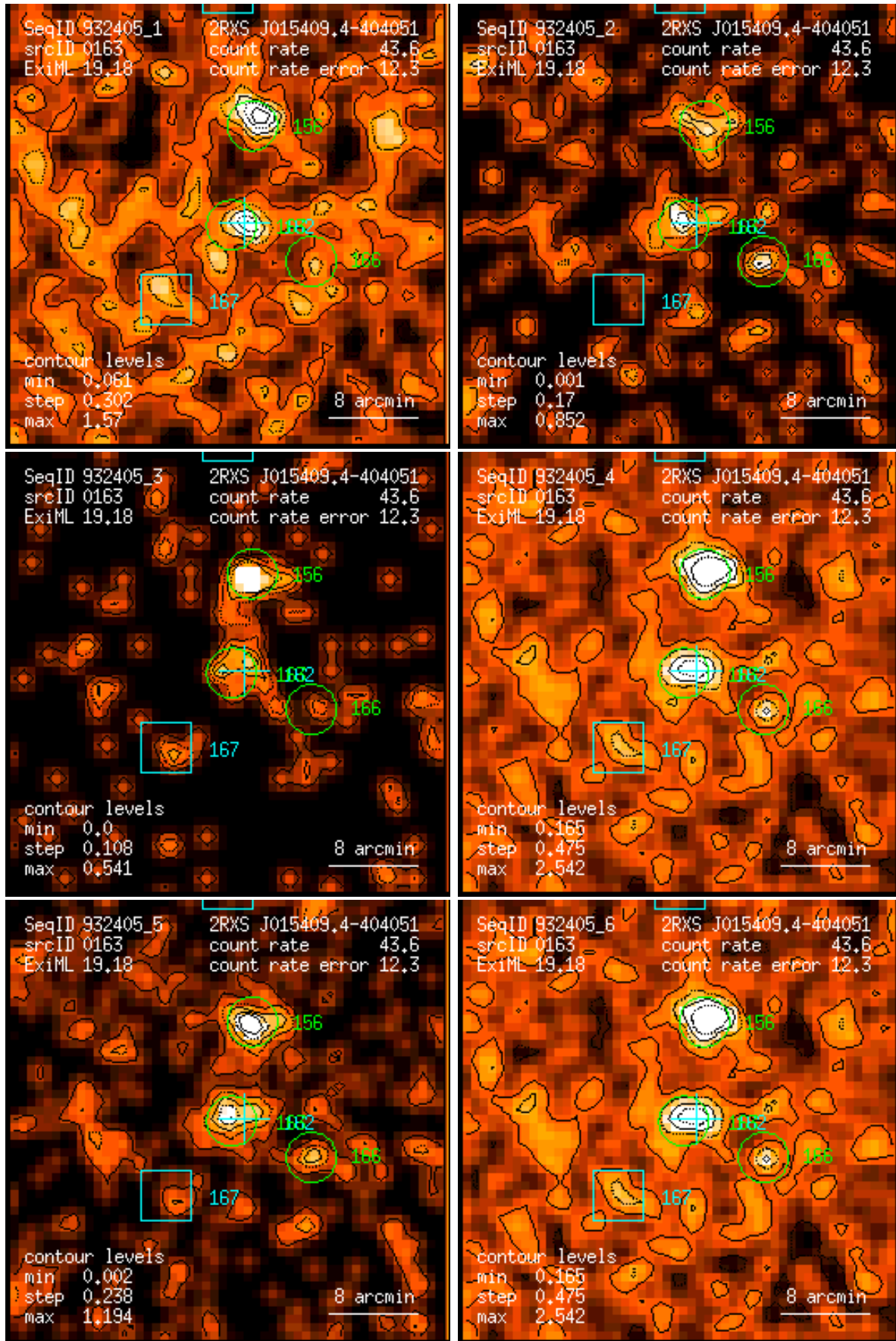
Figure 163: RASS 932405: detection 0163: band rate images, Gaussian filter: (1) PSPC channels 11 – 41, (2) 52 – 90, (3) 91 – 201, (4) 11 – 235, (5) 52 – 201, (6) 11 – 201. Broad band rates in counts/ks. Band rate contour levels in counts/ks/arcmin 2 .
