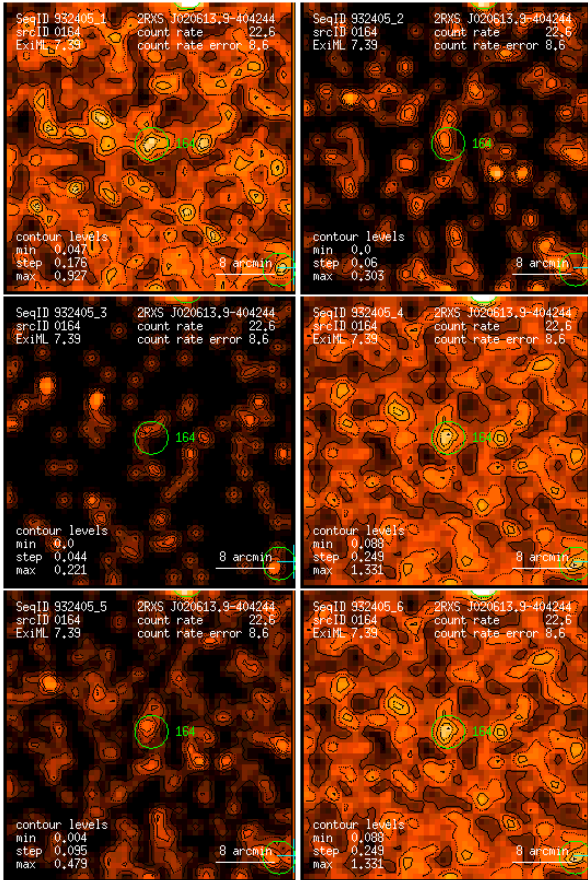
Figure 164: RASS 932405: detection 0164: band rate images, Gaussian filter: (1) PSPC channels 11 – 41, (2) 52 – 90, (3) 91 – 201, (4) 11 – 235, (5) 52 – 201, (6) 11 – 201. Broad band rates in counts/ks. Band rate contour levels in counts/ks/arcmin 2 .
