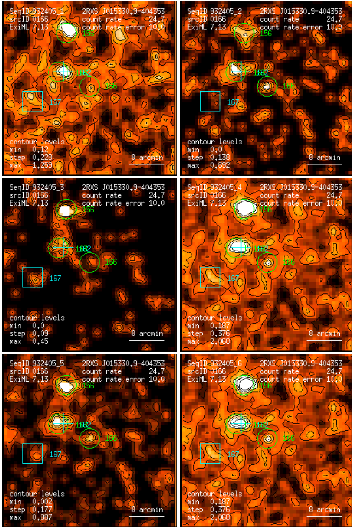
Figure 166: RASS 932405: detection 0166: band rate images, Gaussian filter: (1) PSPC channels 11 – 41, (2) 52 – 90, (3) 91 – 201, (4) 11 – 235, (5) 52 – 201, (6) 11 – 201. Broad band rates in counts/ks. Band rate contour levels in counts/ks/arcmin 2 .
