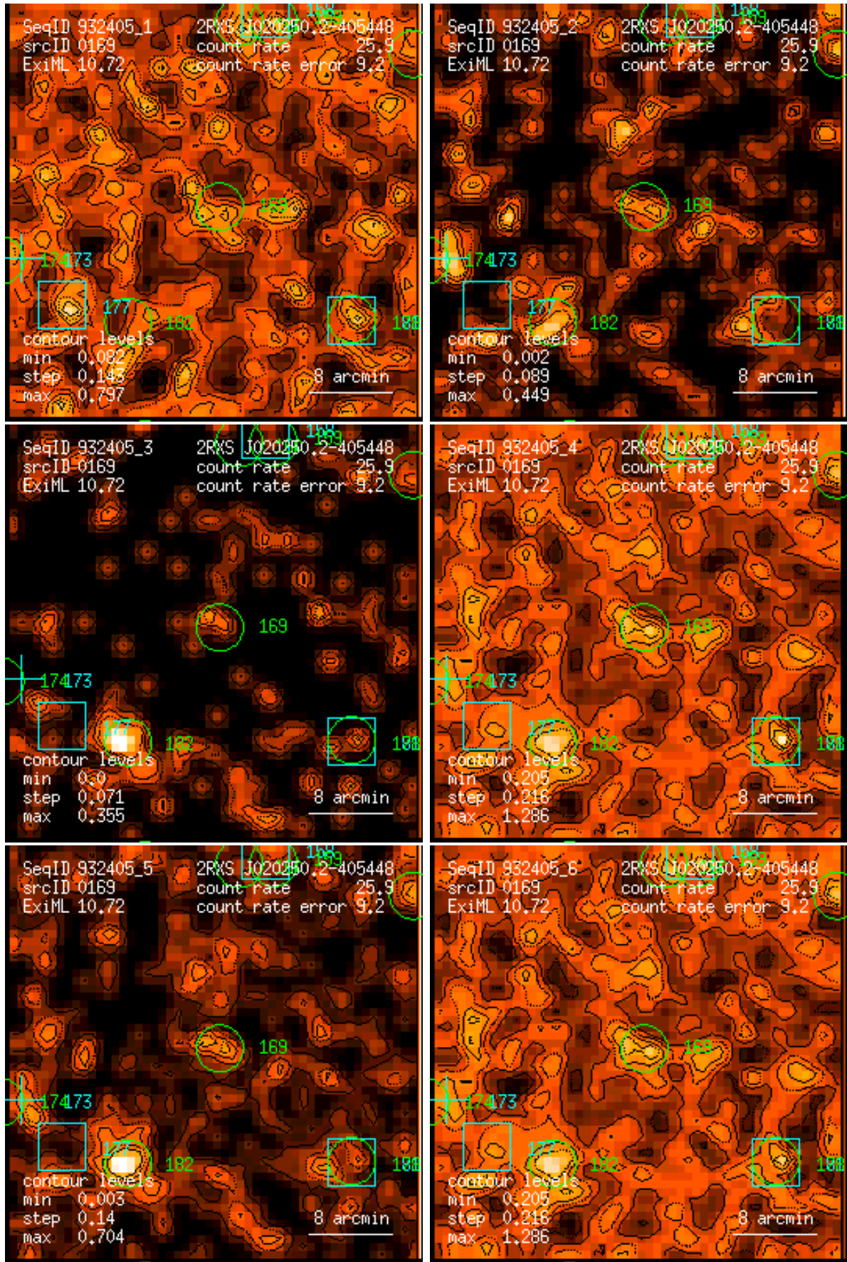
Figure 169: RASS 932405: detection 0169: band rate images, Gaussian filter: (1) PSPC channels 11 – 41, (2) 52 – 90, (3) 91 – 201, (4) 11 – 235, (5) 52 – 201, (6) 11 – 201. Broad band rates in counts/ks. Band rate contour levels in counts/ks/arcmin 2 .
