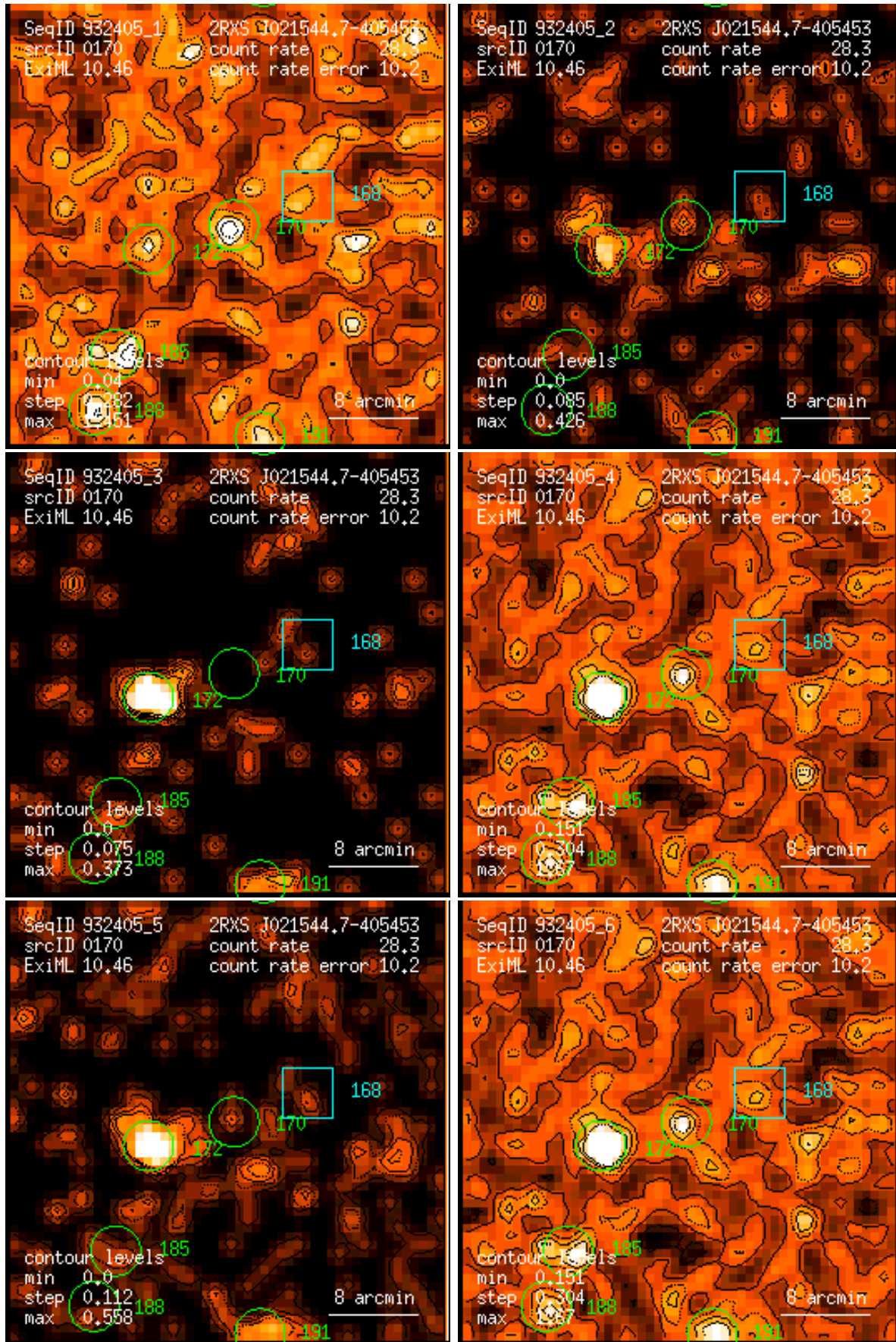
Figure 170: RASS 932405: detection 0170: band rate images, Gaussian filter: (1) PSPC channels 11 – 41, (2) 52 – 90, (3) 91 – 201, (4) 11 – 235, (5) 52 – 201, (6) 11 – 201. Broad band rates in counts/ks. Band rate contour levels in counts/ks/arcmin 2 .
