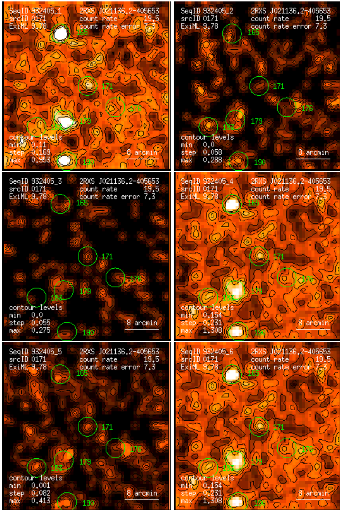
Figure 171: RASS 932405: detection 0171: band rate images, Gaussian filter: (1) PSPC channels 11 – 41, (2) 52 – 90, (3) 91 – 201, (4) 11 – 235, (5) 52 – 201, (6) 11 – 201. Broad band rates in counts/ks. Band rate contour levels in counts/ks/arcmin 2 .
