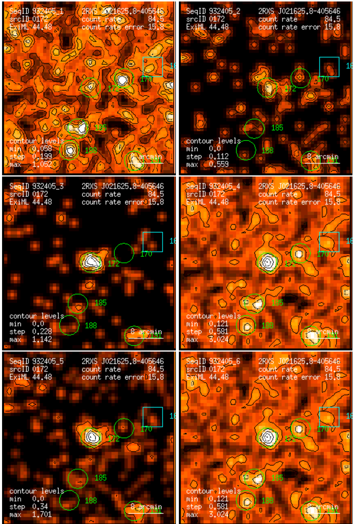
Figure 172: RASS 932405: detection 0172: band rate images, Gaussian filter: (1) PSPC channels 11 – 41, (2) 52 – 90, (3) 91 – 201, (4) 11 – 235, (5) 52 – 201, (6) 11 – 201. Broad band rates in counts/ks. Band rate contour levels in counts/ks/arcmin 2 .
