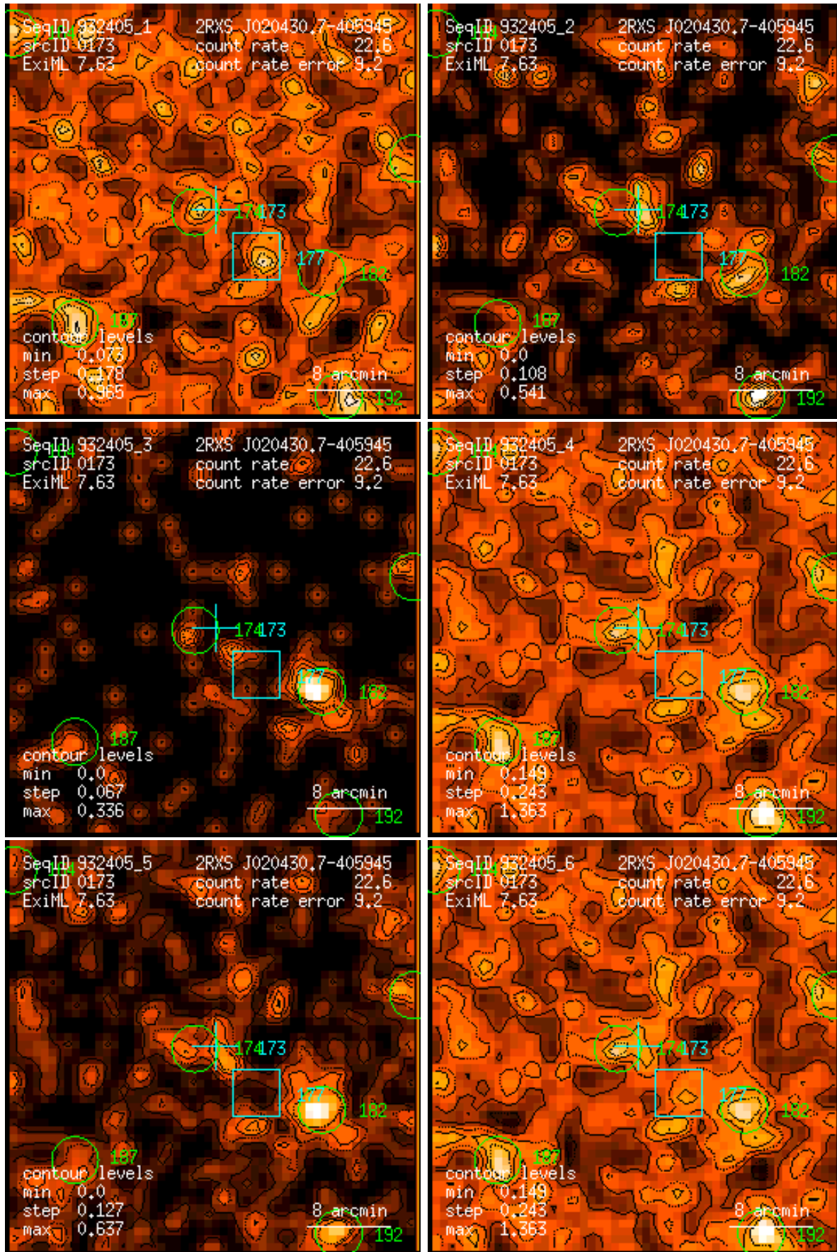
Figure 173: RASS 932405: detection 0173: band rate images, Gaussian filter: (1) PSPC channels 11 – 41, (2) 52 – 90, (3) 91 – 201, (4) 11 – 235, (5) 52 – 201, (6) 11 – 201. Broad band rates in counts/ks. Band rate contour levels in counts/ks/arcmin 2 .
