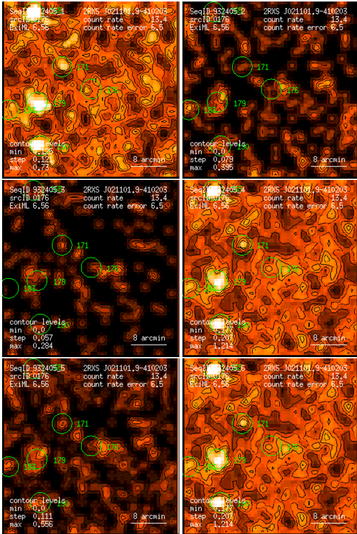
Figure 176: RASS 932405: detection 0176: band rate images, Gaussian filter: (1) PSPC channels 11 – 41, (2) 52 – 90, (3) 91 – 201, (4) 11 – 235, (5) 52 – 201, (6) 11 – 201. Broad band rates in counts/ks. Band rate contour levels in counts/ks/arcmin 2 .
