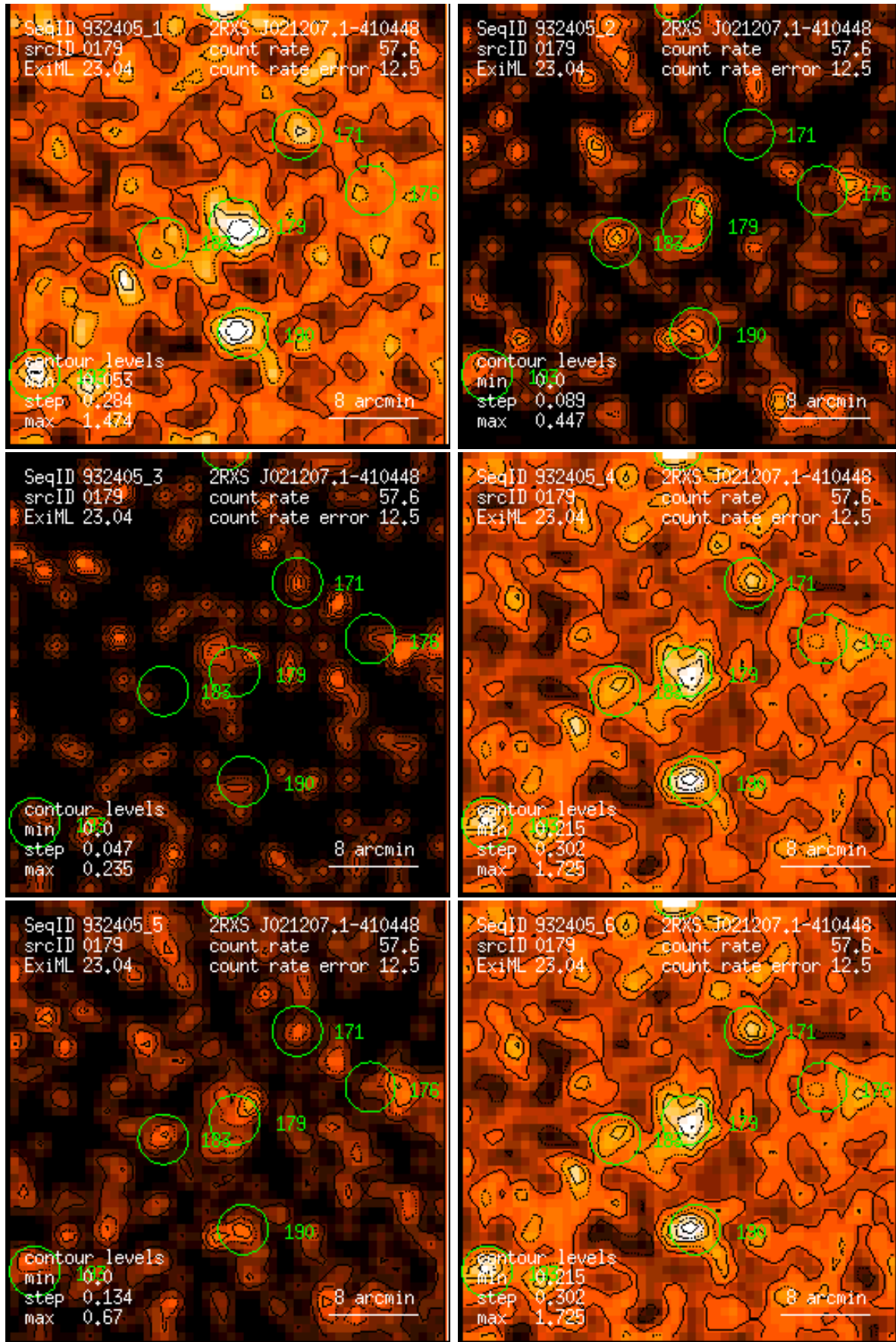
Figure 179: RASS 932405: detection 0179: band rate images, Gaussian filter: (1) PSPC channels 11 – 41, (2) 52 – 90, (3) 91 – 201, (4) 11 – 235, (5) 52 – 201, (6) 11 – 201. Broad band rates in counts/ks. Band rate contour levels in counts/ks/arcmin 2 .
