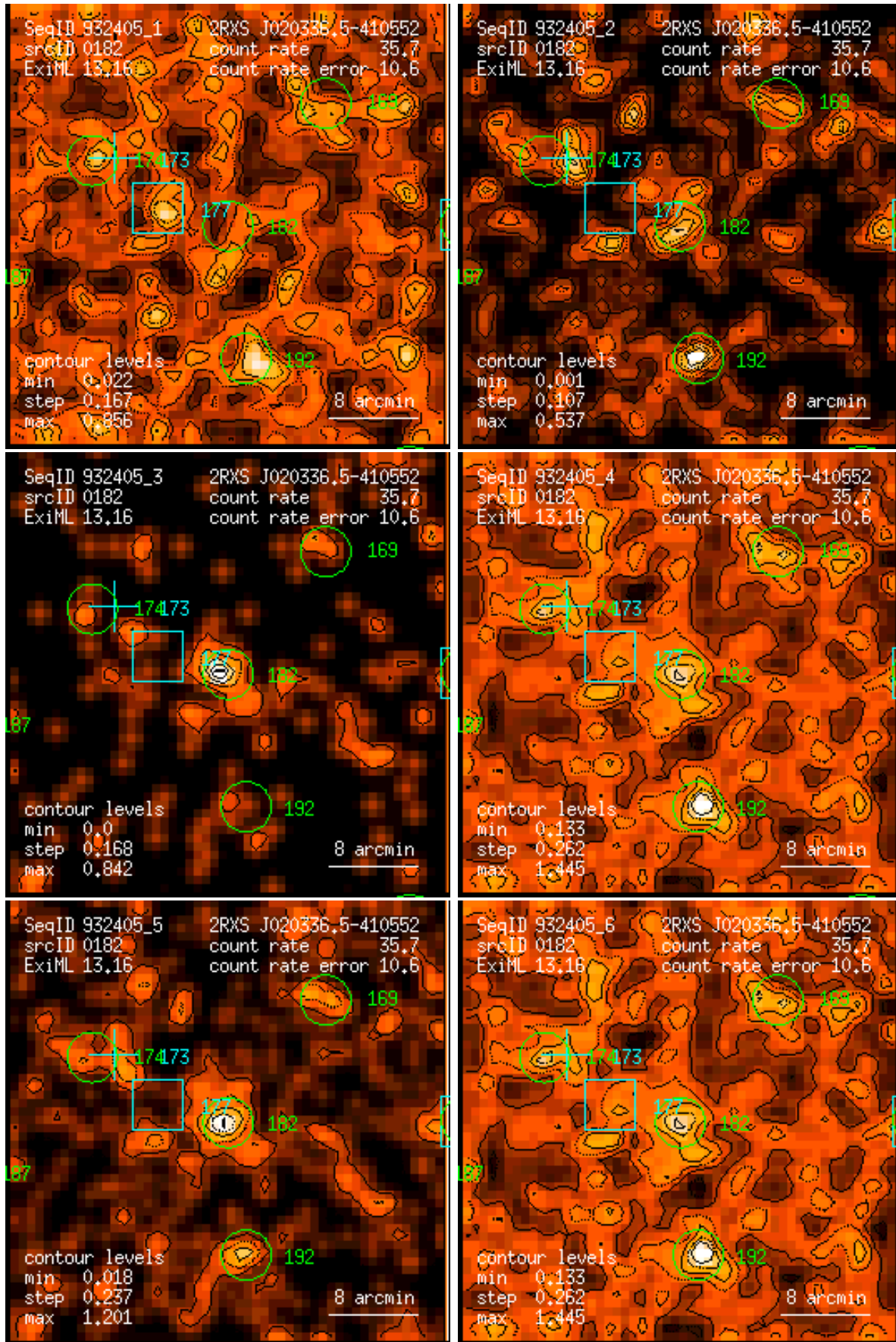
Figure 182: RASS 932405: detection 0182: band rate images, Gaussian filter: (1) PSPC channels 11 – 41, (2) 52 – 90, (3) 91 – 201, (4) 11 – 235, (5) 52 – 201, (6) 11 – 201. Broad band rates in counts/ks. Band rate contour levels in counts/ks/arcmin 2 .
