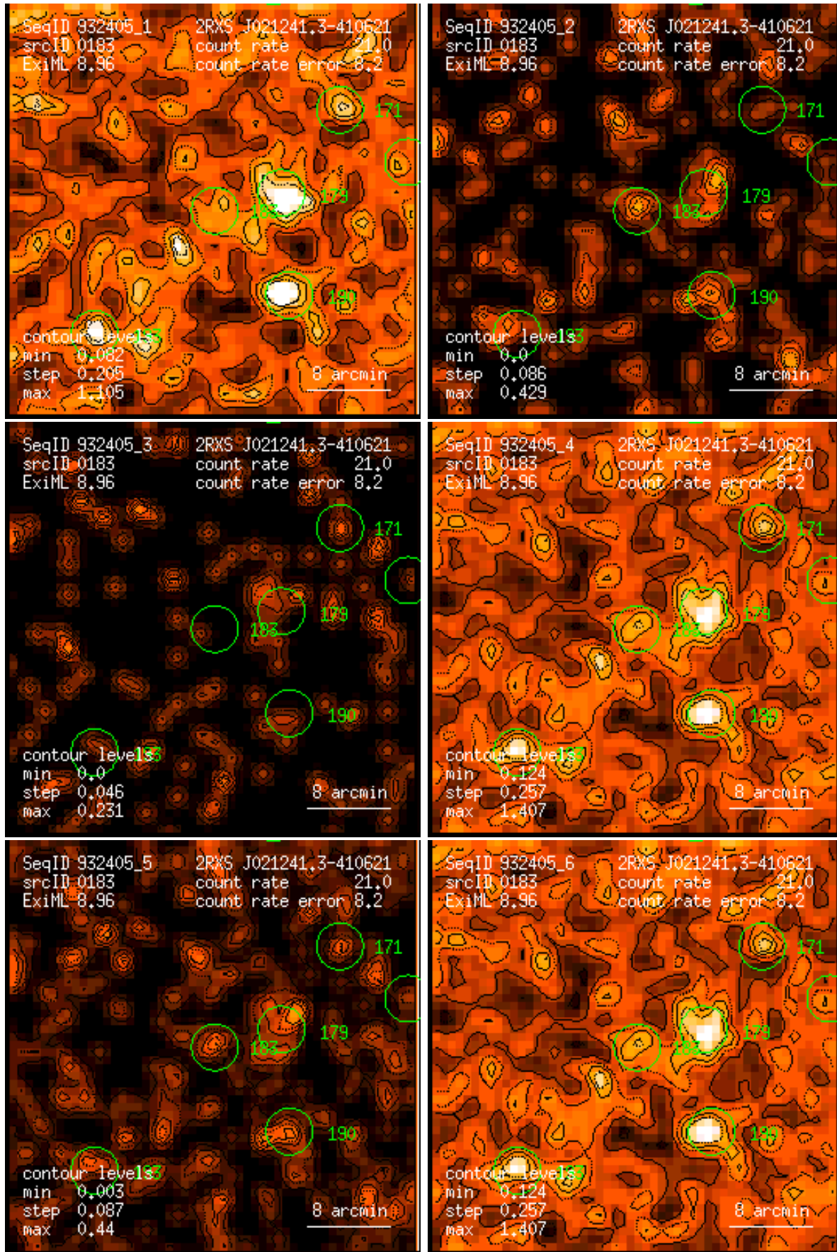
Figure 183: RASS 932405: detection 0183: band rate images, Gaussian filter: (1) PSPC channels 11 – 41, (2) 52 – 90, (3) 91 – 201, (4) 11 – 235, (5) 52 – 201, (6) 11 – 201. Broad band rates in counts/ks. Band rate contour levels in counts/ks/arcmin 2 .
