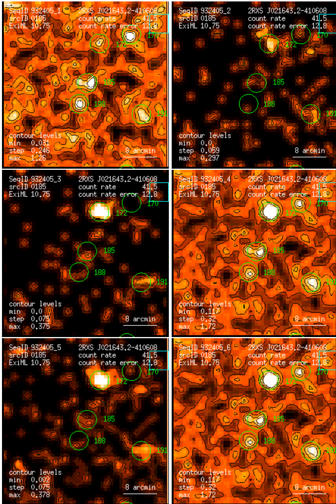
Figure 185: RASS 932405: detection 0185: band rate images, Gaussian filter: (1) PSPC channels 11 – 41, (2) 52 – 90, (3) 91 – 201, (4) 11 – 235, (5) 52 – 201, (6) 11 – 201. Broad band rates in counts/ks. Band rate contour levels in counts/ks/arcmin 2 .
