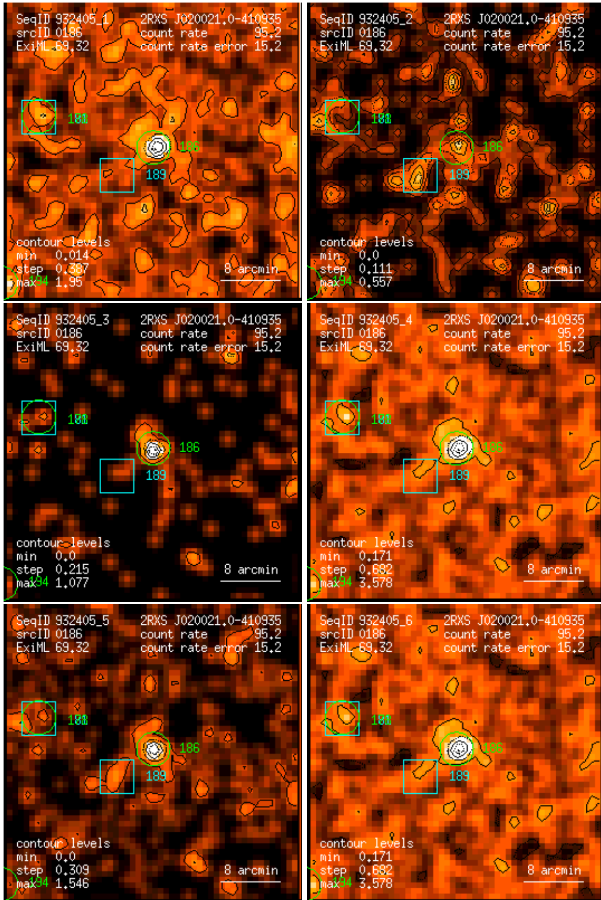
Figure 186: RASS 932405: detection 0186: band rate images, Gaussian filter: (1) PSPC channels 11 – 41, (2) 52 – 90, (3) 91 – 201, (4) 11 – 235, (5) 52 – 201, (6) 11 – 201. Broad band rates in counts/ks. Band rate contour levels in counts/ks/arcmin 2 .
