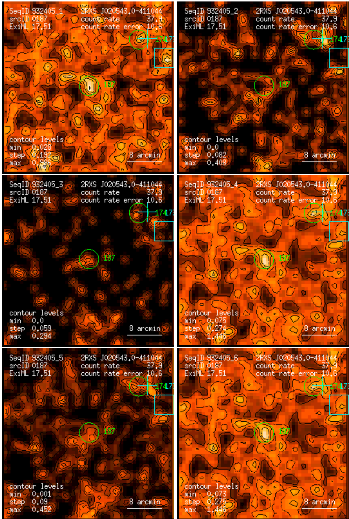
Figure 187: RASS 932405: detection 0187: band rate images, Gaussian filter: (1) PSPC channels 11 – 41, (2) 52 – 90, (3) 91 – 201, (4) 11 – 235, (5) 52 – 201, (6) 11 – 201. Broad band rates in counts/ks. Band rate contour levels in counts/ks/arcmin 2 .
